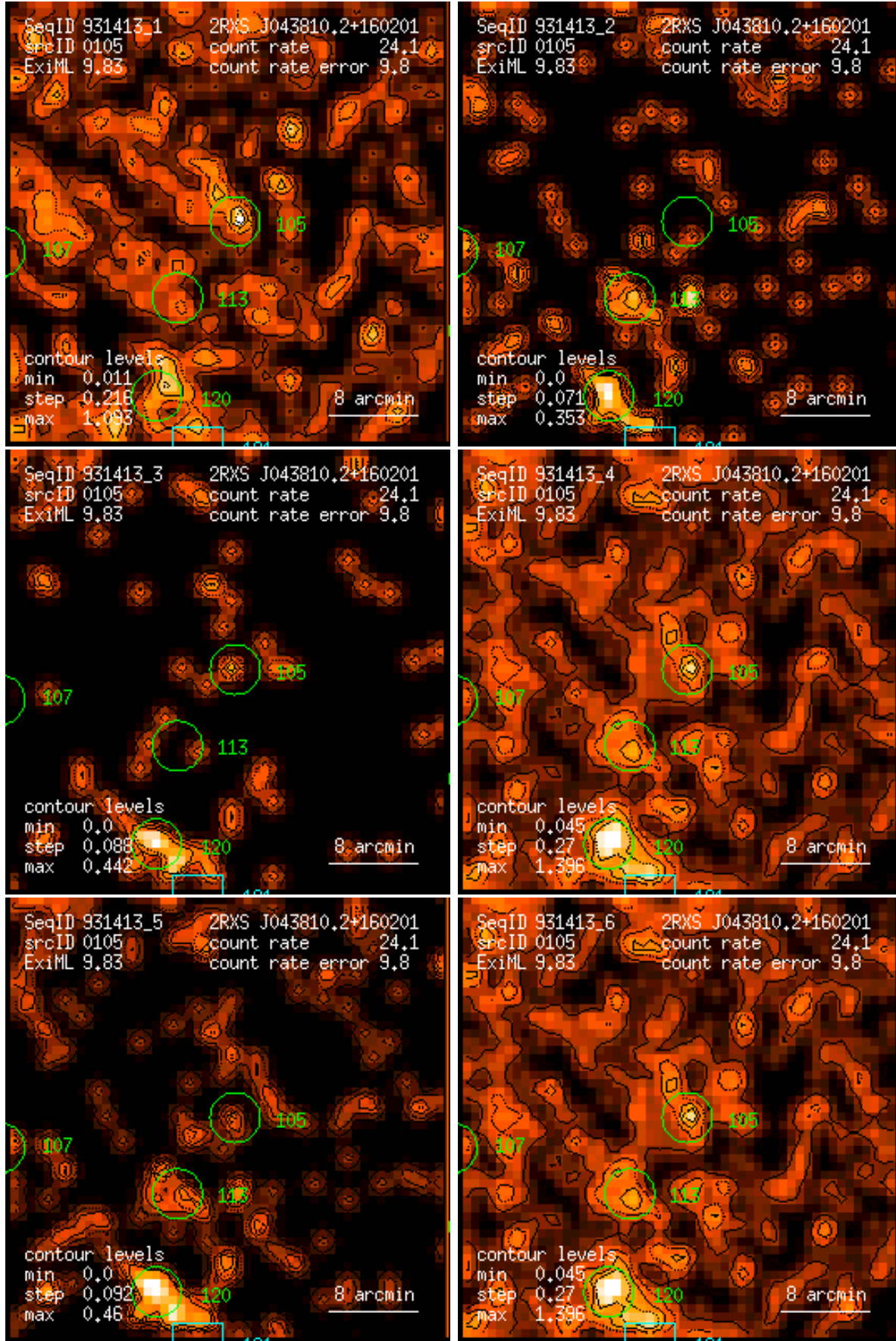
Figure 105: RASS 931413: detection 0105: band rate images, Gaussian filter: (1) PSPC channels 11 – 41, (2) 52 – 90, (3) 91 – 201, (4) 11 – 235, (5) 52 – 201, (6) 11 – 201. Broad band rates in counts/ks. Band rate contour levels in counts/ks/arcmin 2 .
