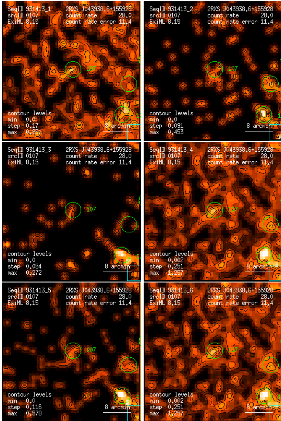
Figure 107: RASS 931413: detection 0107: band rate images, Gaussian filter: (1) PSPC channels 11 – 41, (2) 52 – 90, (3) 91 – 201, (4) 11 – 235, (5) 52 – 201, (6) 11 – 201. Broad band rates in counts/ks. Band rate contour levels in counts/ks/arcmin 2 .
