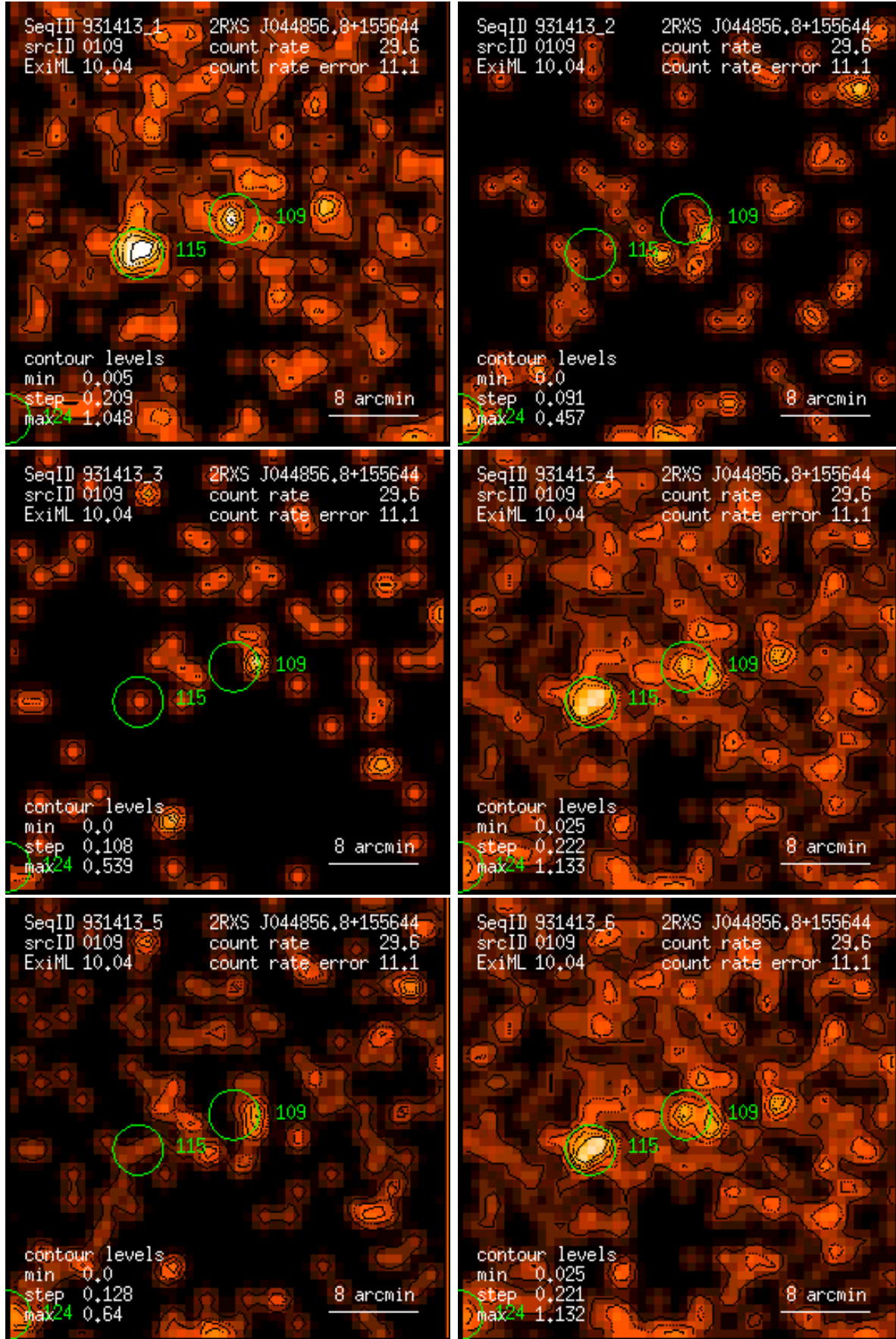
Figure 109: RASS 931413: detection 0109: band rate images, Gaussian filter: (1) PSPC channels 11 – 41, (2) 52 – 90, (3) 91 – 201, (4) 11 – 235, (5) 52 – 201, (6) 11 – 201. Broad band rates in counts/ks. Band rate contour levels in counts/ks/arcmin 2 .
