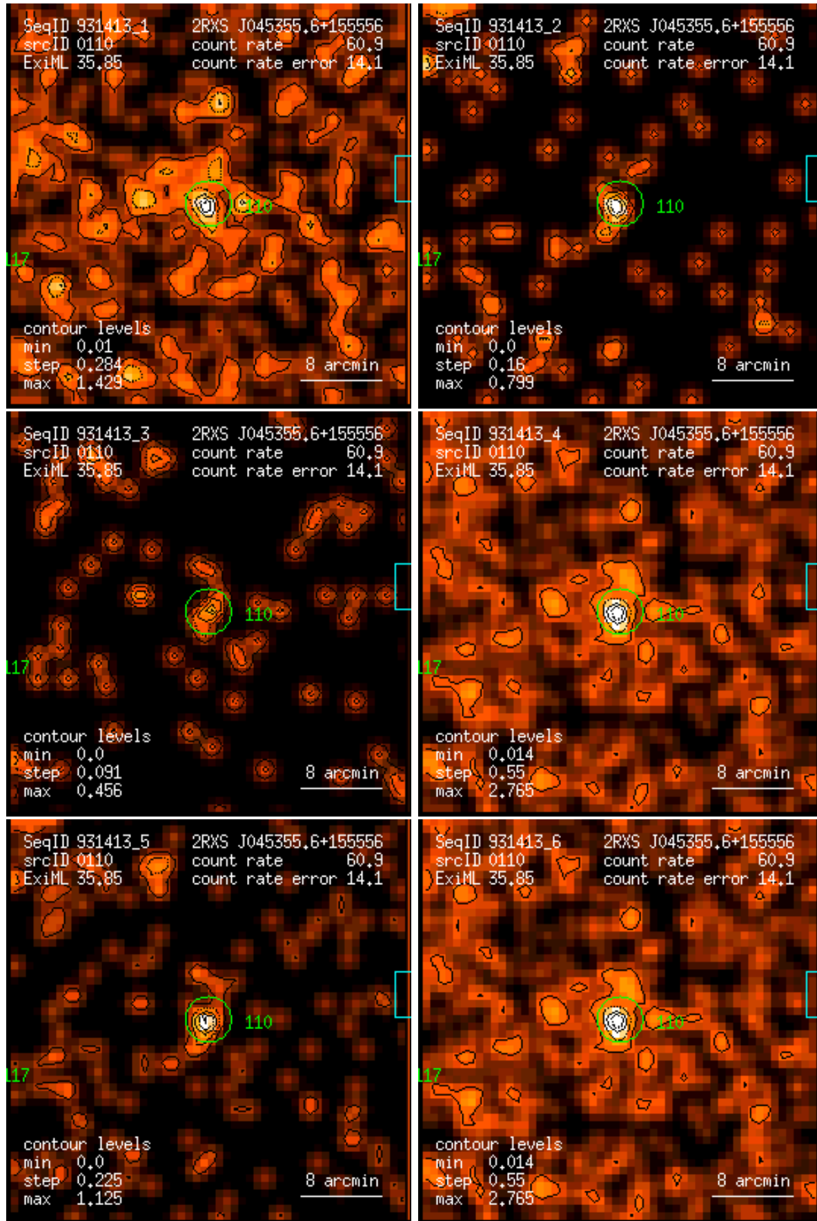
Figure 110: RASS 931413: detection 0110: band rate images, Gaussian filter: (1) PSPC channels 11 – 41, (2) 52 – 90, (3) 91 – 201, (4) 11 – 235, (5) 52 – 201, (6) 11 – 201. Broad band rates in counts/ks. Band rate contour levels in counts/ks/arcmin 2 .
