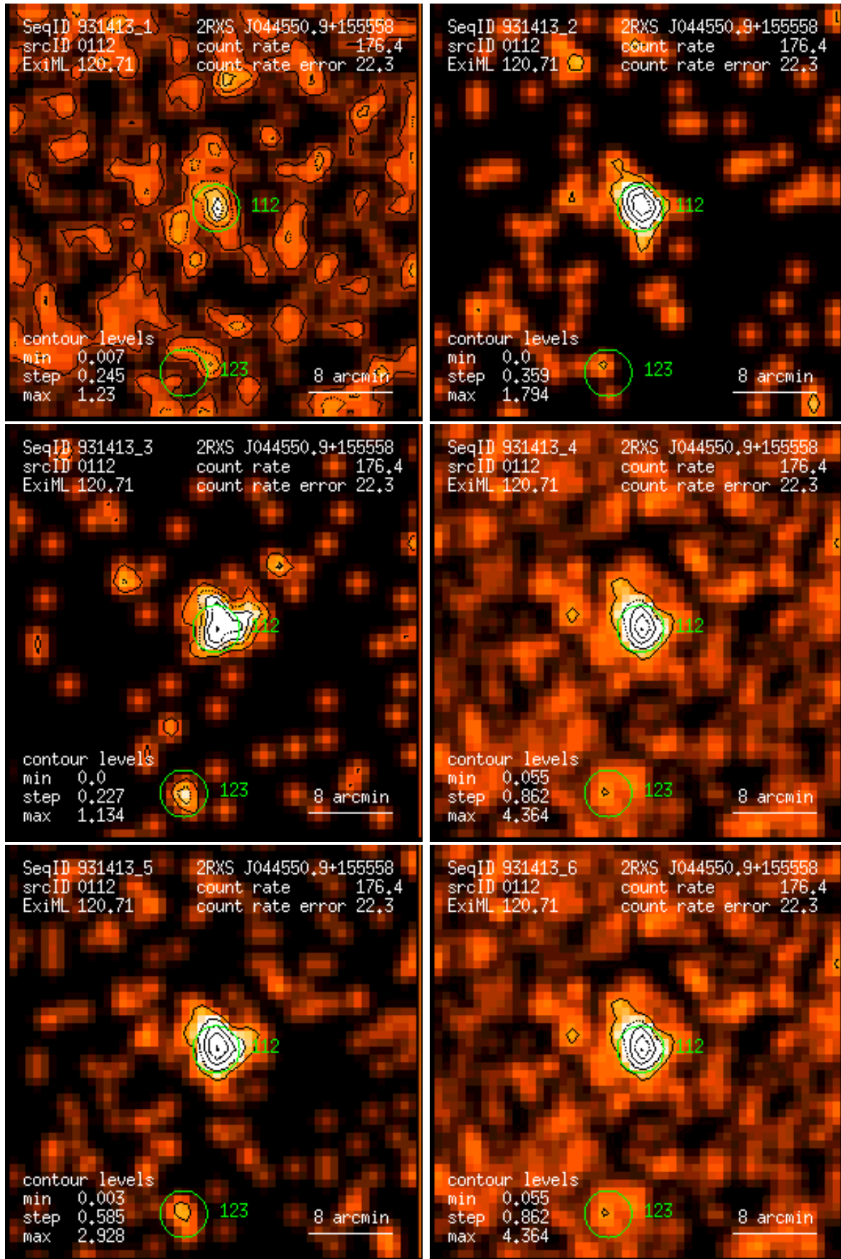
Figure 112: RASS 931413: detection 0112: band rate images, Gaussian filter: (1) PSPC channels 11 – 41, (2) 52 – 90, (3) 91 – 201, (4) 11 – 235, (5) 52 – 201, (6) 11 – 201. Broad band rates in counts/ks. Band rate contour levels in counts/ks/arcmin 2 .
