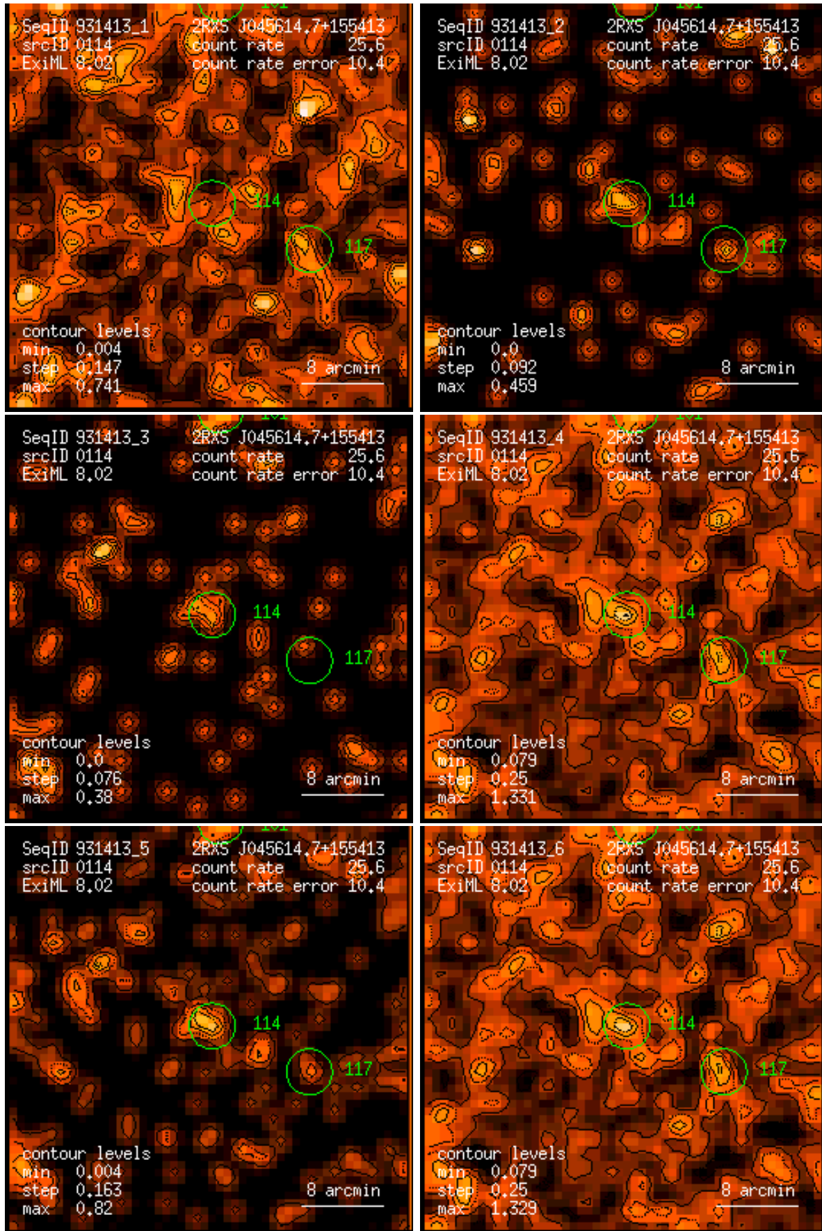
Figure 114: RASS 931413: detection 0114: band rate images, Gaussian filter: (1) PSPC channels 11 – 41, (2) 52 – 90, (3) 91 – 201, (4) 11 – 235, (5) 52 – 201, (6) 11 – 201. Broad band rates in counts/ks. Band rate contour levels in counts/ks/arcmin 2 .
