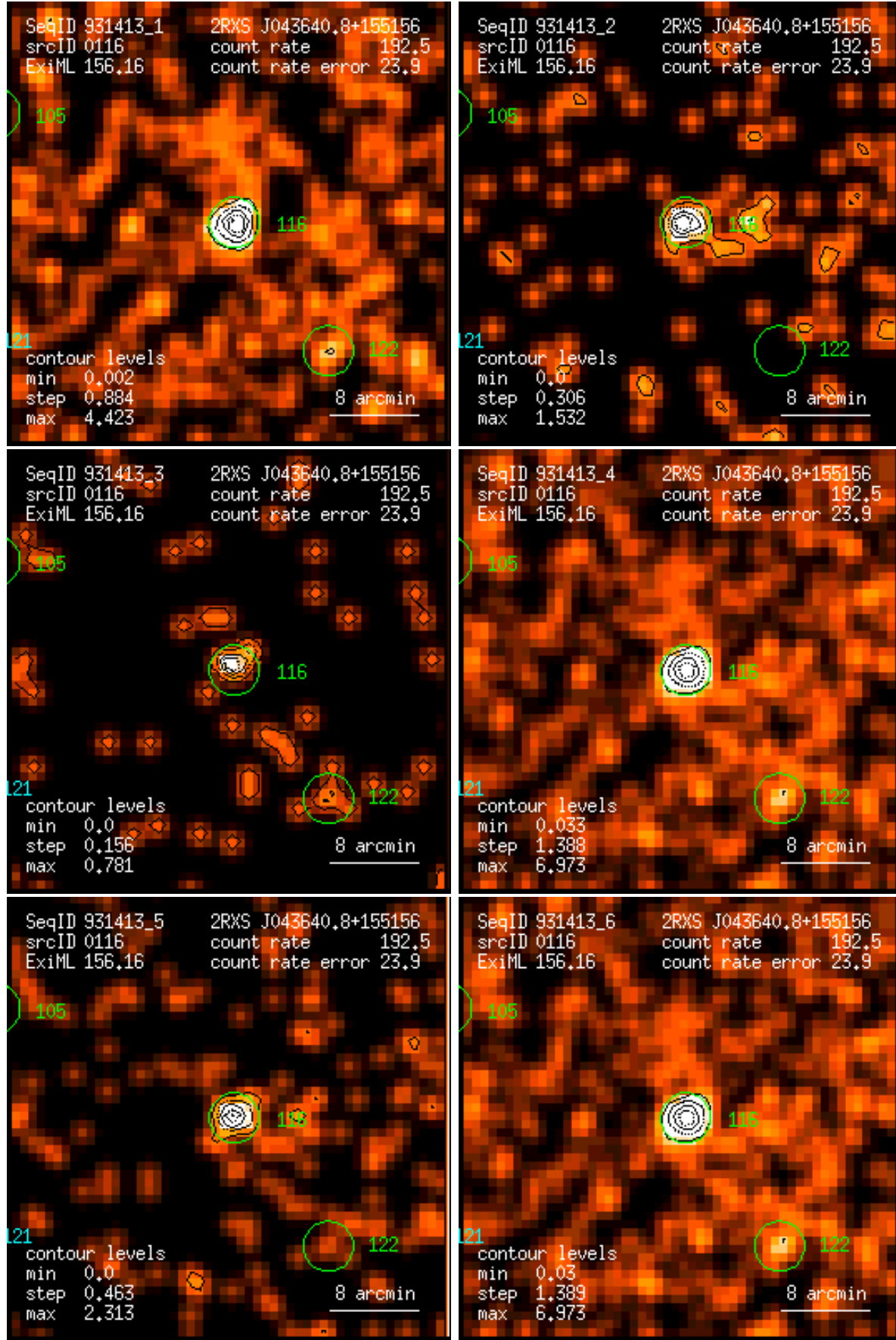
Figure 116: RASS 931413: detection 0116: band rate images, Gaussian filter: (1) PSPC channels 11 – 41, (2) 52 – 90, (3) 91 – 201, (4) 11 – 235, (5) 52 – 201, (6) 11 – 201. Broad band rates in counts/ks. Band rate contour levels in counts/ks/arcmin 2 .
