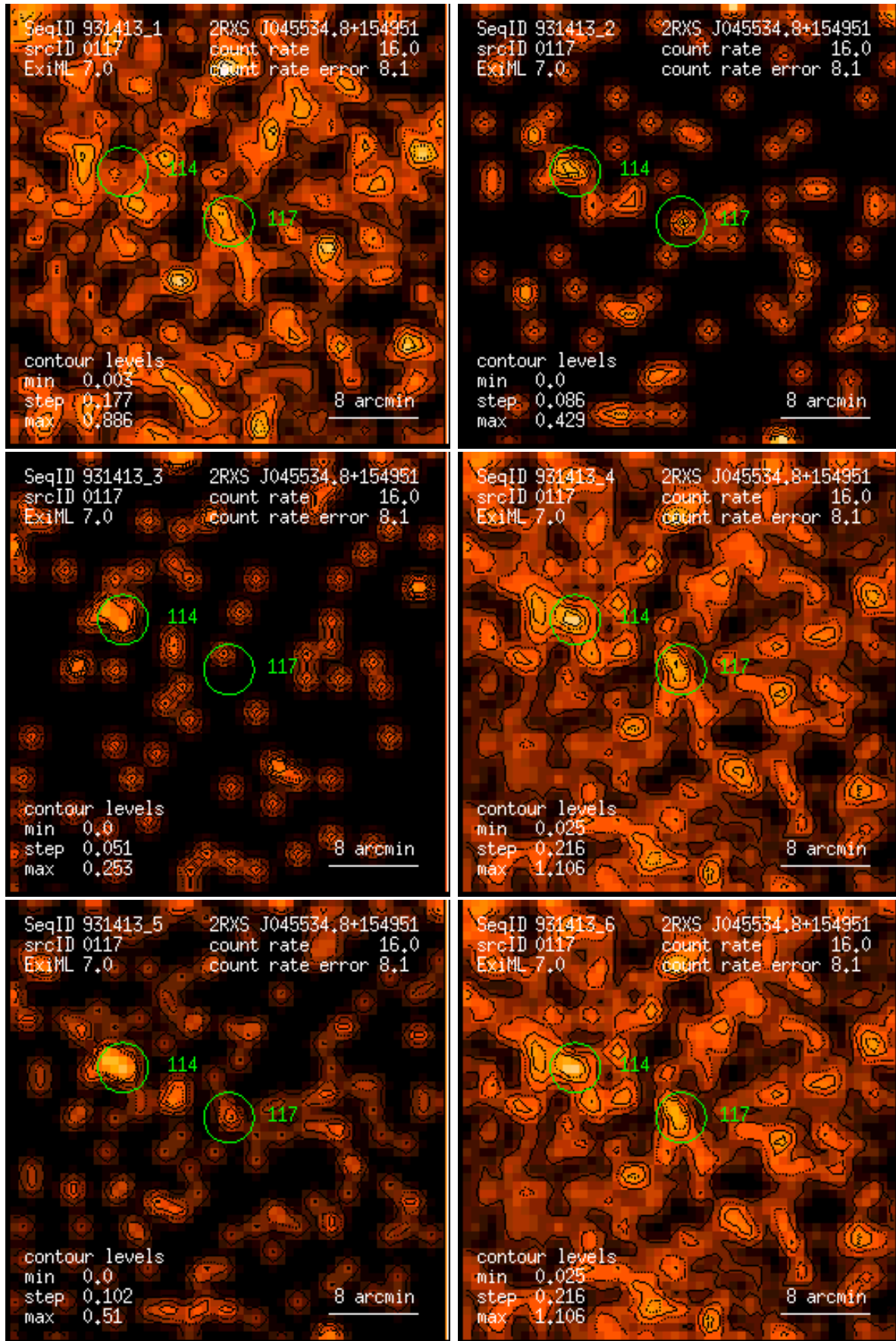
Figure 117: RASS 931413: detection 0117: band rate images, Gaussian filter: (1) PSPC channels 11 – 41, (2) 52 – 90, (3) 91 – 201, (4) 11 – 235, (5) 52 – 201, (6) 11 – 201. Broad band rates in counts/ks. Band rate contour levels in counts/ks/arcmin 2 .
