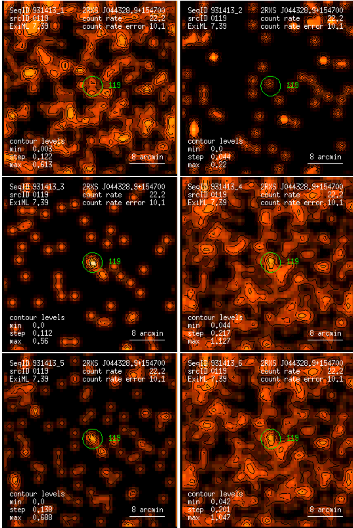
Figure 119: RASS 931413: detection 0119: band rate images, Gaussian filter: (1) PSPC channels 11 – 41, (2) 52 – 90, (3) 91 – 201, (4) 11 – 235, (5) 52 – 201, (6) 11 – 201. Broad band rates in counts/ks. Band rate contour levels in counts/ks/arcmin 2 .
