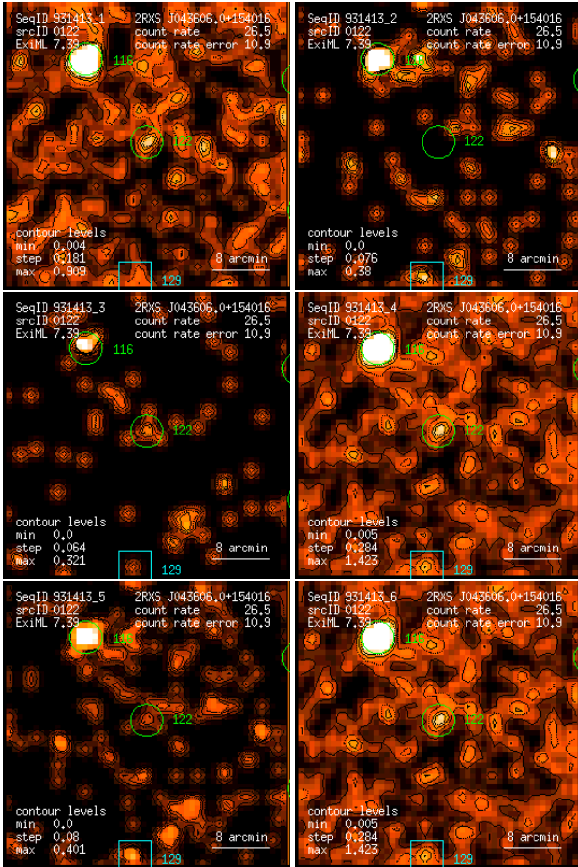
Figure 122: RASS 931413: detection 0122: band rate images, Gaussian filter: (1) PSPC channels 11 – 41, (2) 52 – 90, (3) 91 – 201, (4) 11 – 235, (5) 52 – 201, (6) 11 – 201. Broad band rates in counts/ks. Band rate contour levels in counts/ks/arcmin 2 .
