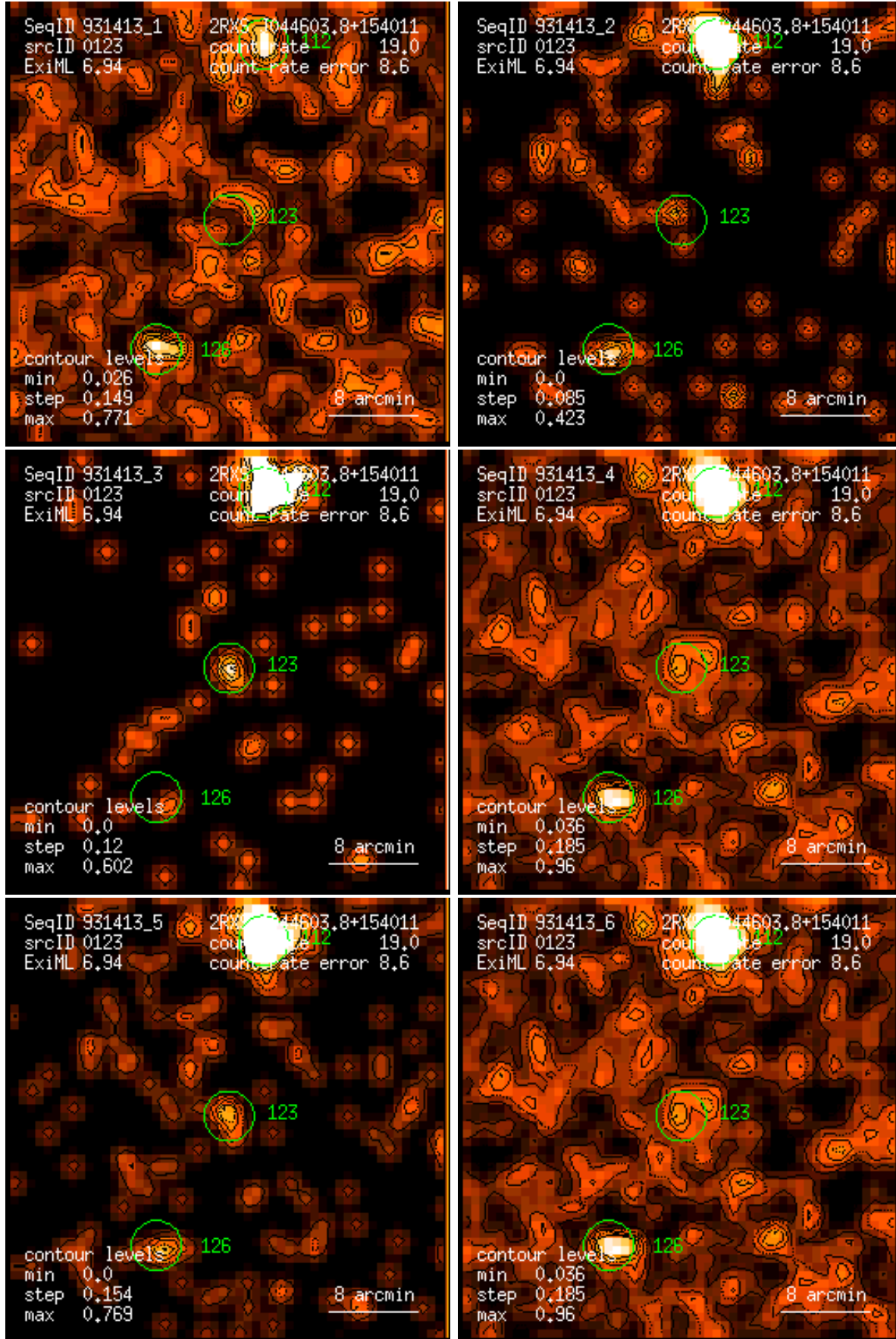
Figure 123: RASS 931413: detection 0123: band rate images, Gaussian filter: (1) PSPC channels 11 – 41, (2) 52 – 90, (3) 91 – 201, (4) 11 – 235, (5) 52 – 201, (6) 11 – 201. Broad band rates in counts/ks. Band rate contour levels in counts/ks/arcmin 2 .
