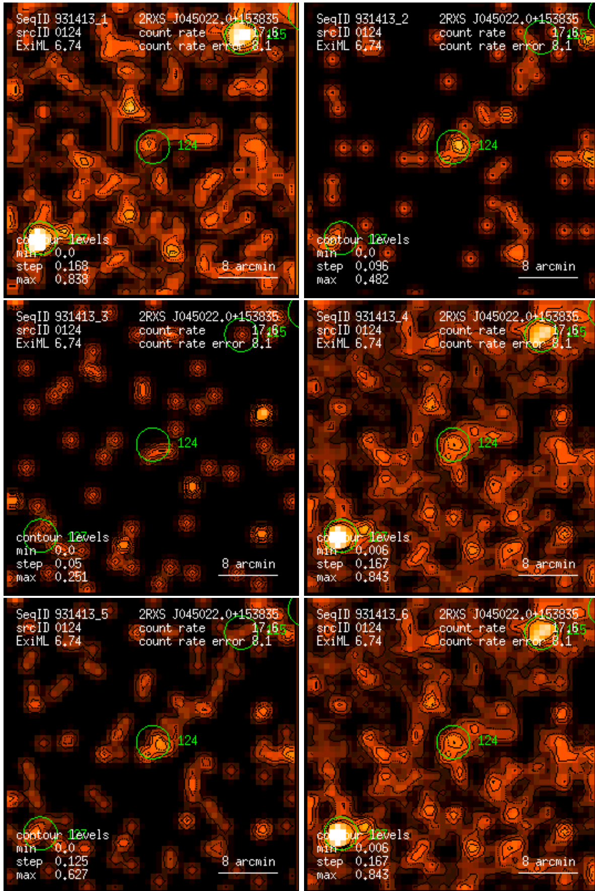
Figure 124: RASS 931413: detection 0124: band rate images, Gaussian filter: (1) PSPC channels 11 – 41, (2) 52 – 90, (3) 91 – 201, (4) 11 – 235, (5) 52 – 201, (6) 11 – 201. Broad band rates in counts/ks. Band rate contour levels in counts/ks/arcmin 2 .
