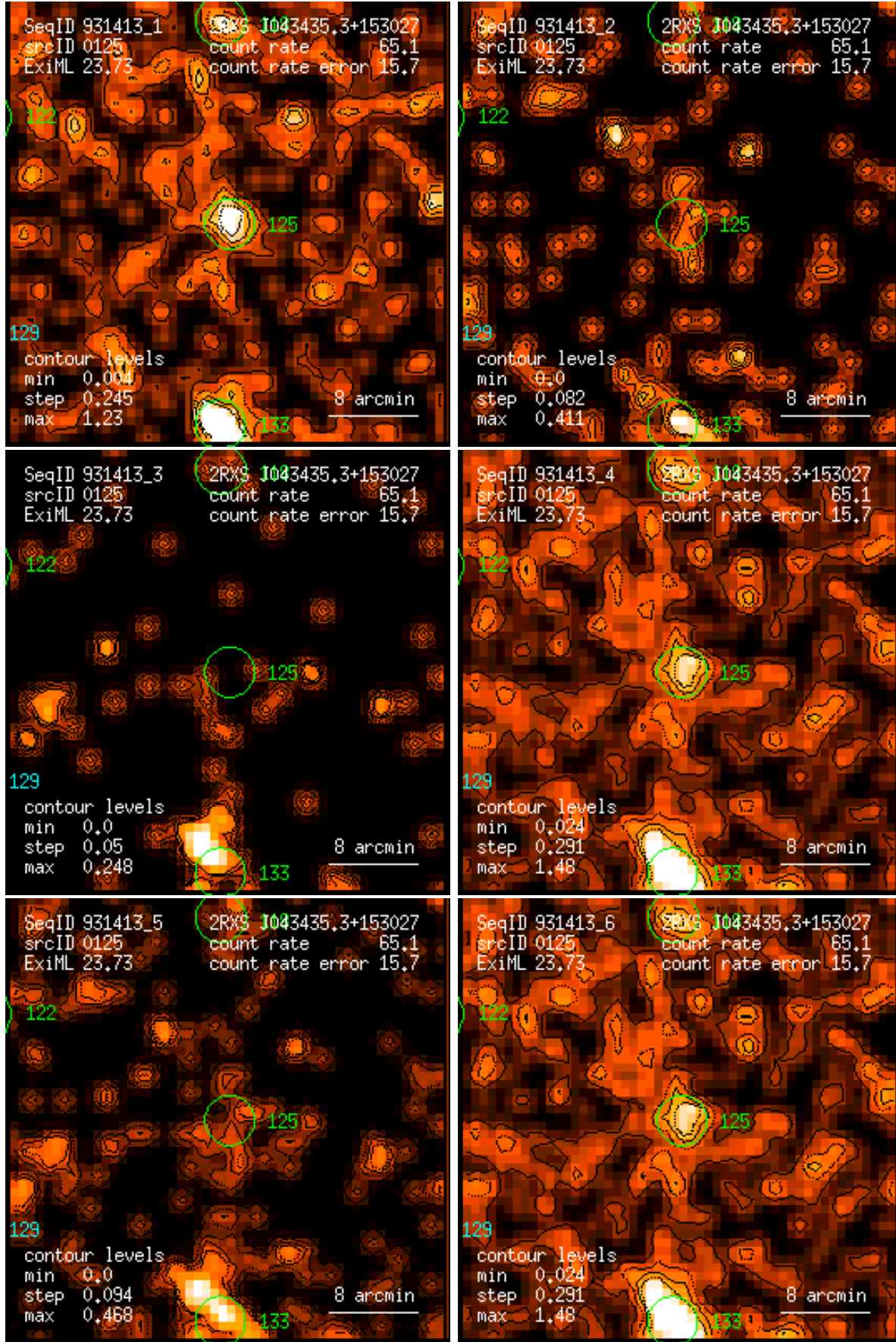
Figure 125: RASS 931413: detection 0125: band rate images, Gaussian filter: (1) PSPC channels 11 – 41, (2) 52 – 90, (3) 91 – 201, (4) 11 – 235, (5) 52 – 201, (6) 11 – 201. Broad band rates in counts/ks. Band rate contour levels in counts/ks/arcmin 2 .
