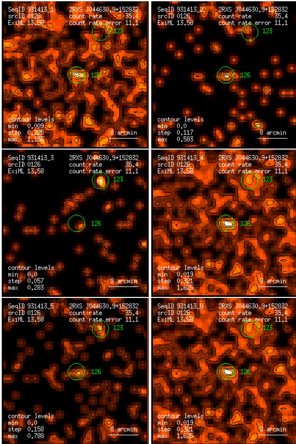
Figure 126: RASS 931413: detection 0126: band rate images, Gaussian filter: (1) PSPC channels 11 – 41, (2) 52 – 90, (3) 91 – 201, (4) 11 – 235, (5) 52 – 201, (6) 11 – 201. Broad band rates in counts/ks. Band rate contour levels in counts/ks/arcmin 2 .
