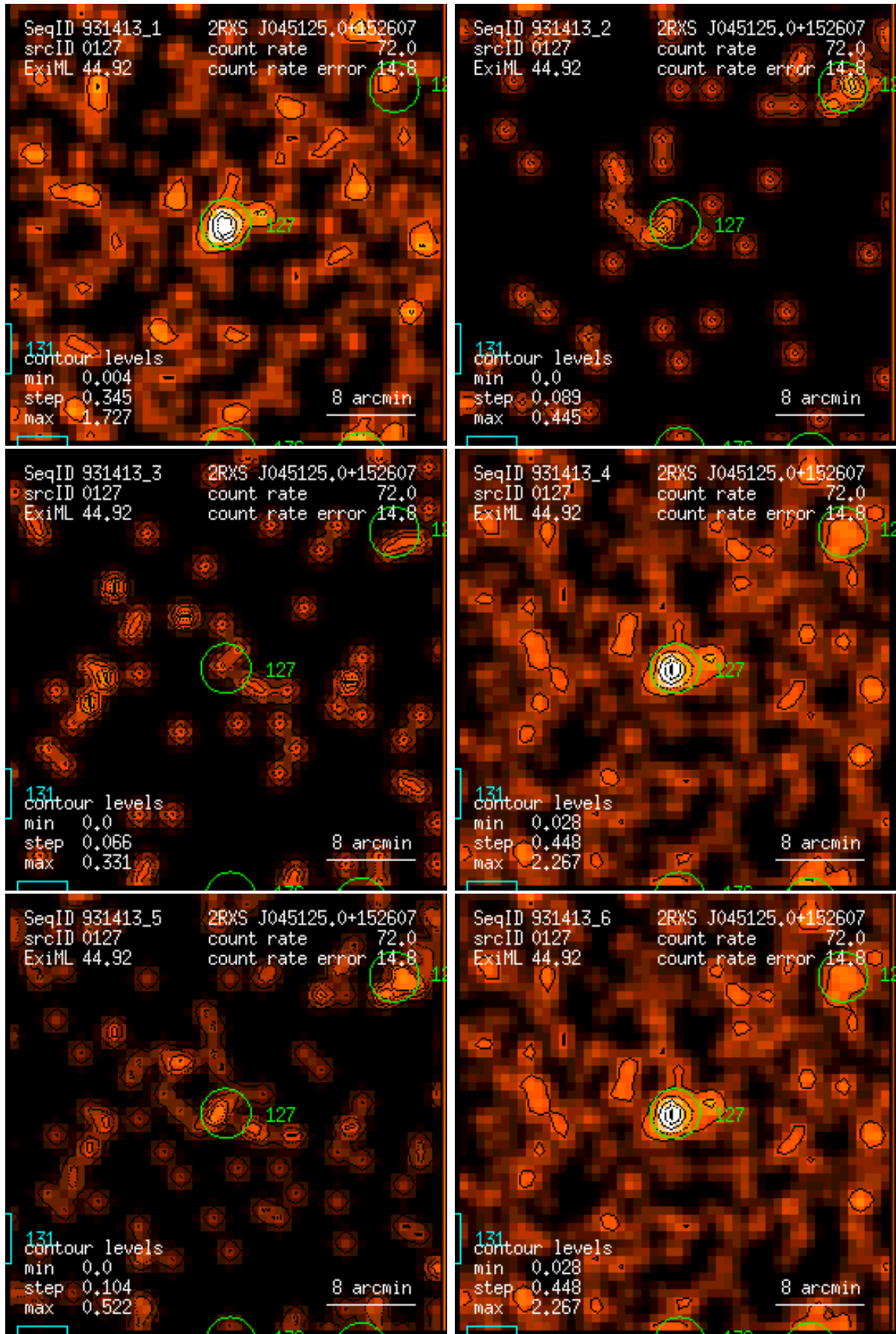
Figure 127: RASS 931413: detection 0127: band rate images, Gaussian filter: (1) PSPC channels 11 – 41, (2) 52 – 90, (3) 91 – 201, (4) 11 – 235, (5) 52 – 201, (6) 11 – 201. Broad band rates in counts/ks. Band rate contour levels in counts/ks/arcmin 2 .
