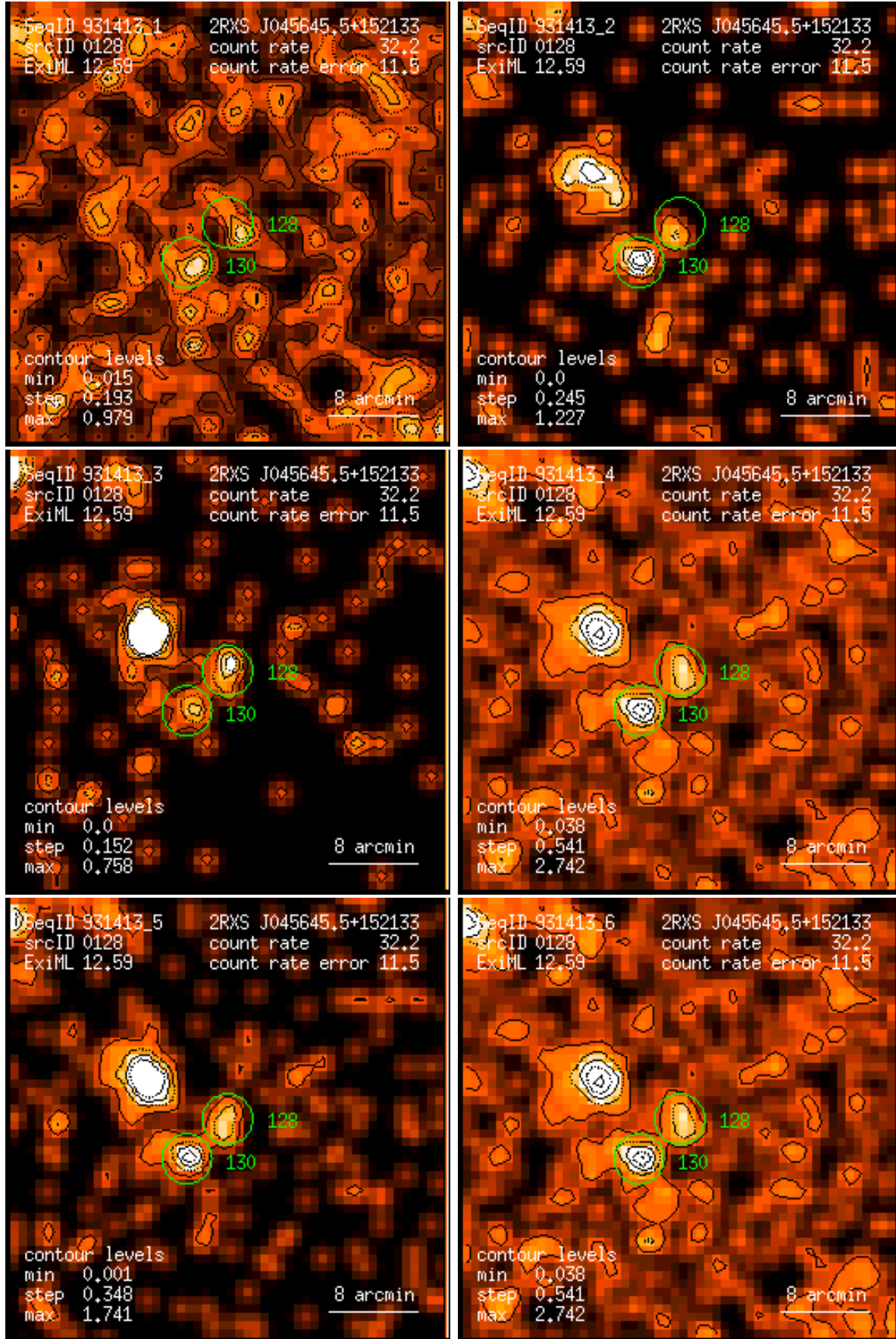
Figure 128: RASS 931413: detection 0128: band rate images, Gaussian filter: (1) PSPC channels 11 – 41, (2) 52 – 90, (3) 91 – 201, (4) 11 – 235, (5) 52 – 201, (6) 11 – 201. Broad band rates in counts/ks. Band rate contour levels in counts/ks/arcmin 2 .
