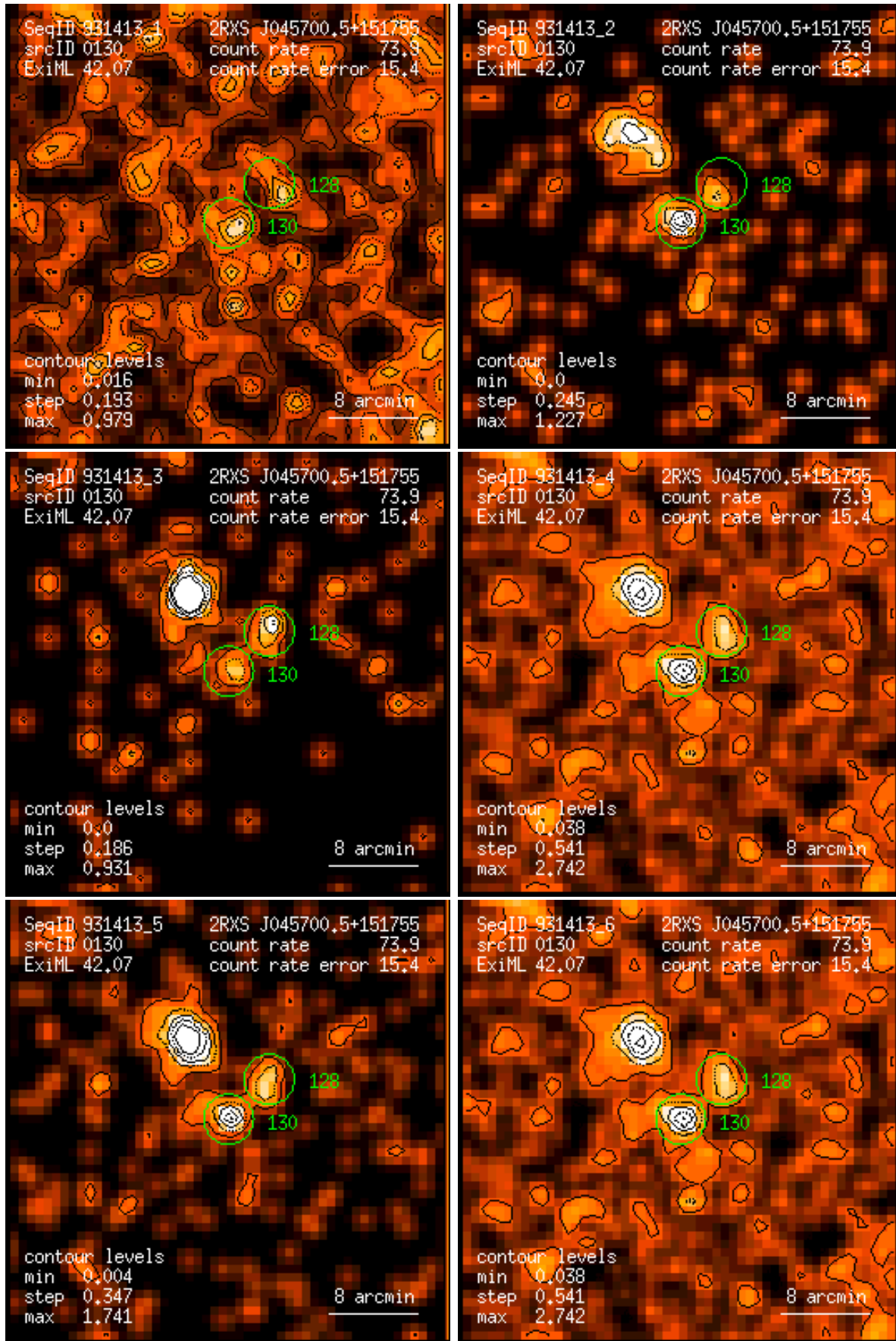
Figure 130: RASS 931413: detection 0130: band rate images, Gaussian filter: (1) PSPC channels 11 – 41, (2) 52 – 90, (3) 91 – 201, (4) 11 – 235, (5) 52 – 201, (6) 11 – 201. Broad band rates in counts/ks. Band rate contour levels in counts/ks/arcmin 2 .
