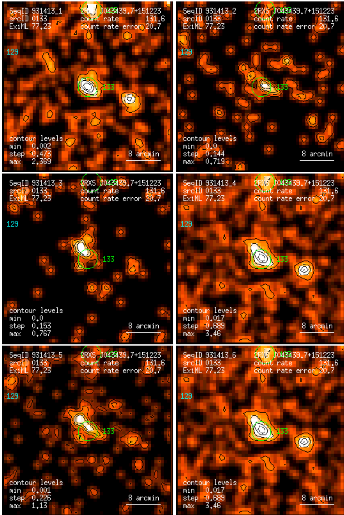
Figure 133: RASS 931413: detection 0133: band rate images, Gaussian filter: (1) PSPC channels 11 – 41, (2) 52 – 90, (3) 91 – 201, (4) 11 – 235, (5) 52 – 201, (6) 11 – 201. Broad band rates in counts/ks. Band rate contour levels in counts/ks/arcmin 2 .
