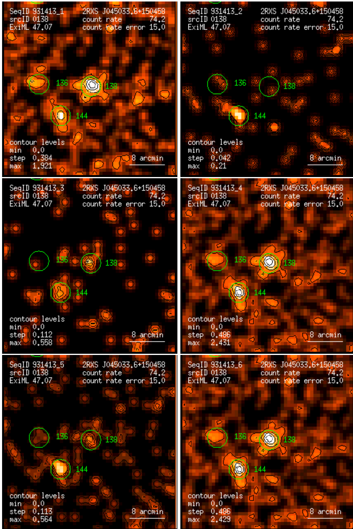
Figure 138: RASS 931413: detection 0138: band rate images, Gaussian filter: (1) PSPC channels 11 – 41, (2) 52 – 90, (3) 91 – 201, (4) 11 – 235, (5) 52 – 201, (6) 11 – 201. Broad band rates in counts/ks. Band rate contour levels in counts/ks/arcmin 2 .
