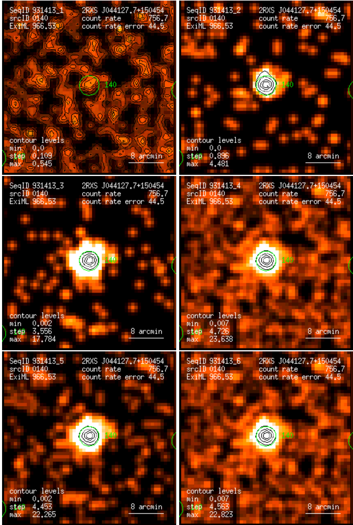
Figure 140: RASS 931413: detection 0140: band rate images, Gaussian filter: (1) PSPC channels 11 – 41, (2) 52 – 90, (3) 91 – 201, (4) 11 – 235, (5) 52 – 201, (6) 11 – 201. Broad band rates in counts/ks. Band rate contour levels in counts/ks/arcmin 2 .
