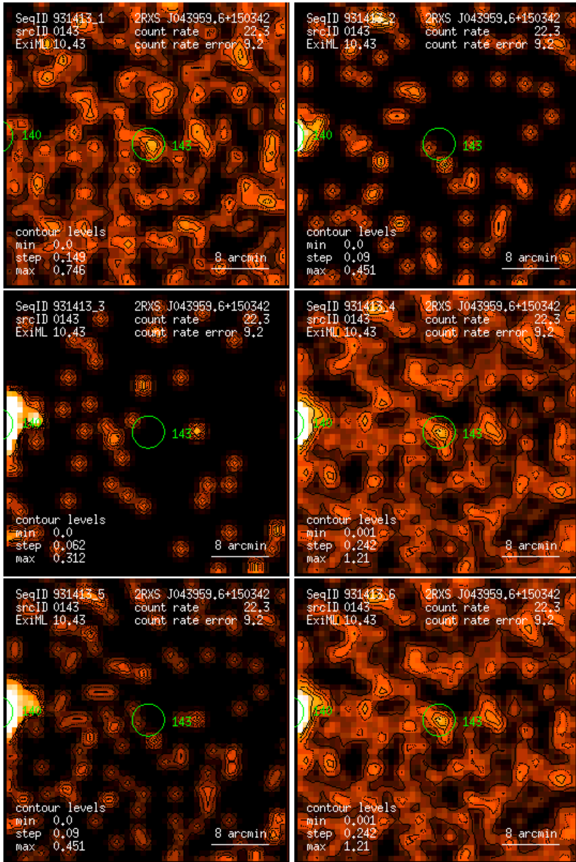
Figure 143: RASS 931413: detection 0143: band rate images, Gaussian filter: (1) PSPC channels 11 – 41, (2) 52 – 90, (3) 91 – 201, (4) 11 – 235, (5) 52 – 201, (6) 11 – 201. Broad band rates in counts/ks. Band rate contour levels in counts/ks/arcmin 2 .
