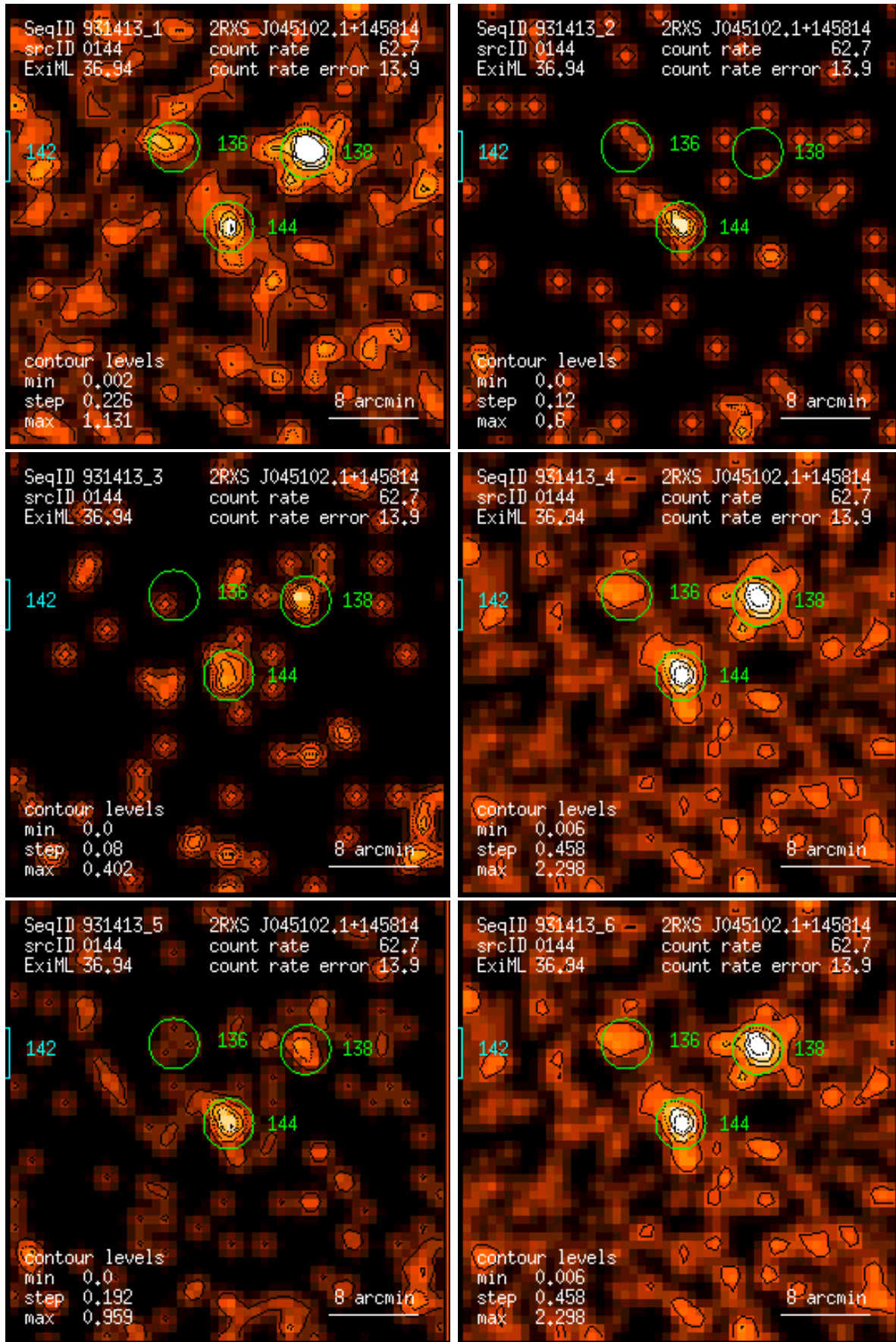
Figure 144: RASS 931413: detection 0144: band rate images, Gaussian filter: (1) PSPC channels 11 – 41, (2) 52 – 90, (3) 91 – 201, (4) 11 – 235, (5) 52 – 201, (6) 11 – 201. Broad band rates in counts/ks. Band rate contour levels in counts/ks/arcmin 2 .
