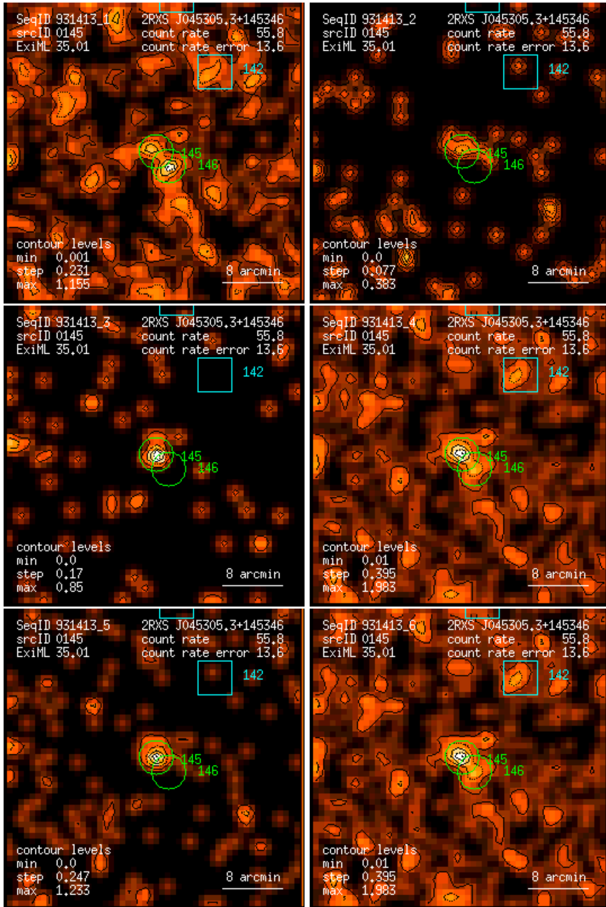
Figure 145: RASS 931413: detection 0145: band rate images, Gaussian filter: (1) PSPC channels 11 – 41, (2) 52 – 90, (3) 91 – 201, (4) 11 – 235, (5) 52 – 201, (6) 11 – 201. Broad band rates in counts/ks. Band rate contour levels in counts/ks/arcmin 2 .
