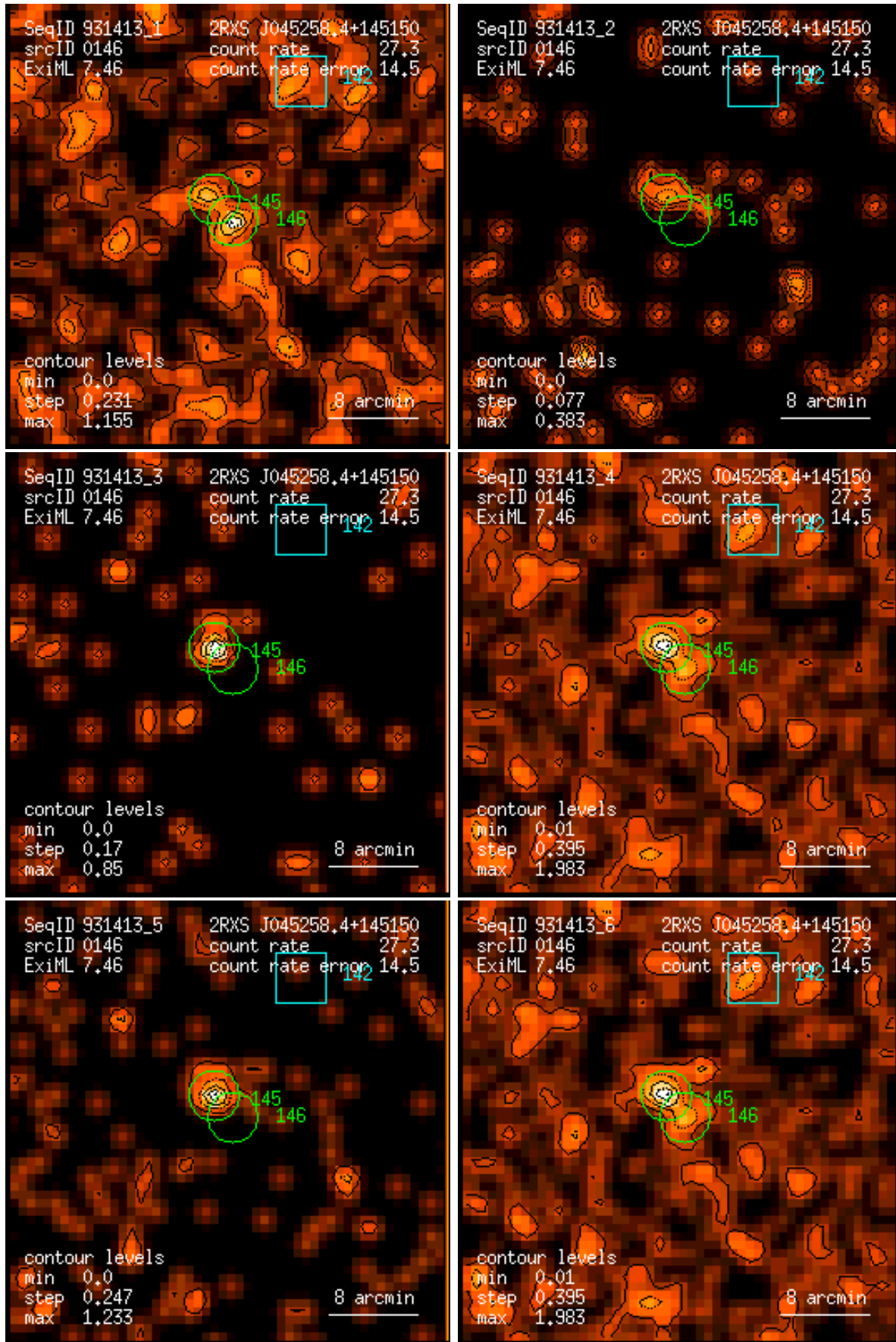
Figure 146: RASS 931413: detection 0146: band rate images, Gaussian filter: (1) PSPC channels 11 – 41, (2) 52 – 90, (3) 91 – 201, (4) 11 – 235, (5) 52 – 201, (6) 11 – 201. Broad band rates in counts/ks. Band rate contour levels in counts/ks/arcmin 2 .
