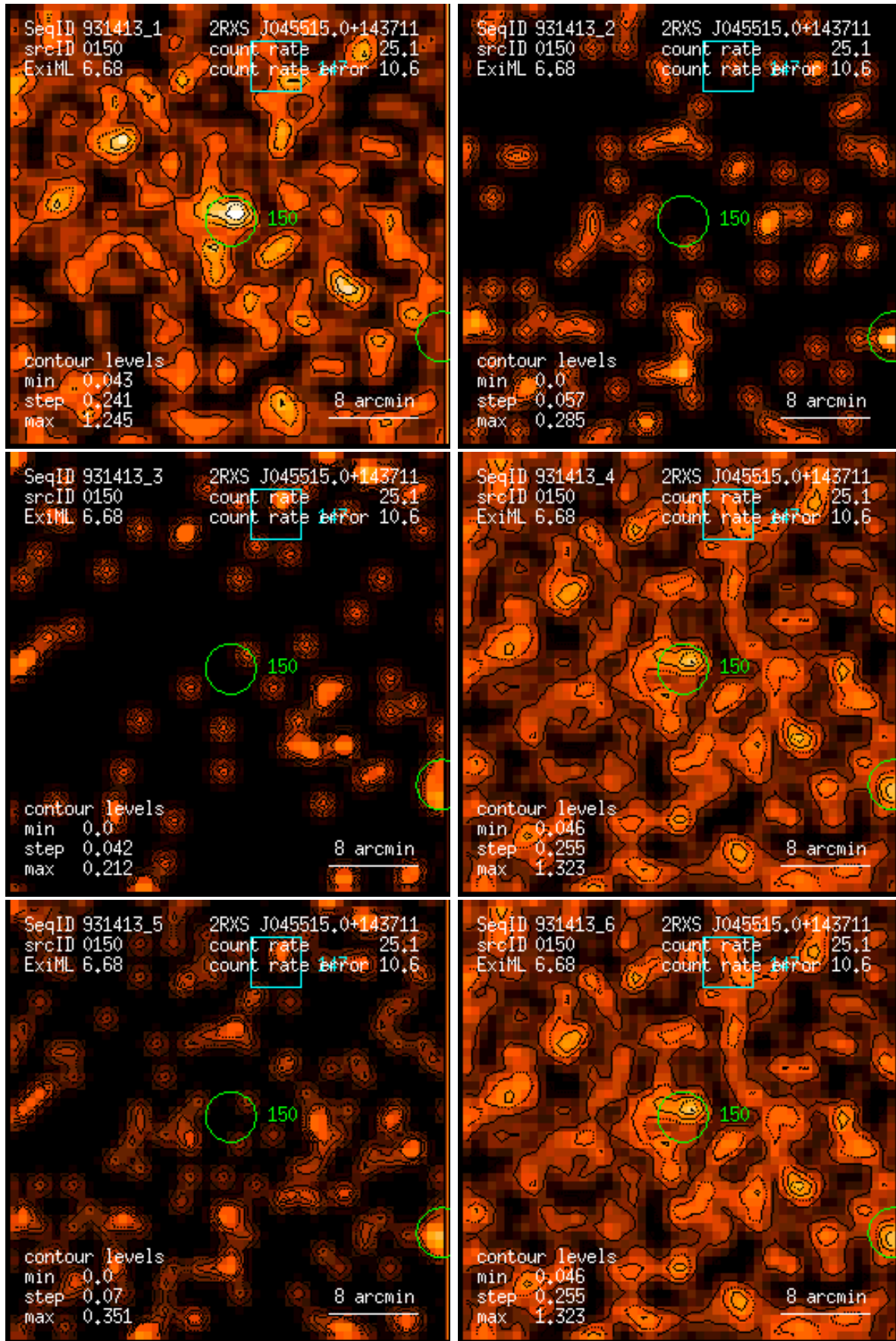
Figure 150: RASS 931413: detection 0150: band rate images, Gaussian filter: (1) PSPC channels 11 – 41, (2) 52 – 90, (3) 91 – 201, (4) 11 – 235, (5) 52 – 201, (6) 11 – 201. Broad band rates in counts/ks. Band rate contour levels in counts/ks/arcmin 2 .
