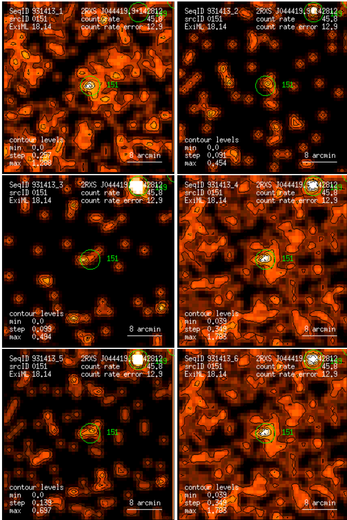
Figure 151: RASS 931413: detection 0151: band rate images, Gaussian filter: (1) PSPC channels 11 – 41, (2) 52 – 90, (3) 91 – 201, (4) 11 – 235, (5) 52 – 201, (6) 11 – 201. Broad band rates in counts/ks. Band rate contour levels in counts/ks/arcmin 2 .
