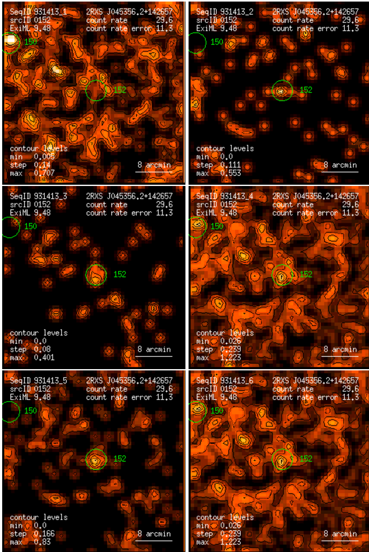
Figure 152: RASS 931413: detection 0152: band rate images, Gaussian filter: (1) PSPC channels 11 – 41, (2) 52 – 90, (3) 91 – 201, (4) 11 – 235, (5) 52 – 201, (6) 11 – 201. Broad band rates in counts/ks. Band rate contour levels in counts/ks/arcmin 2 .
