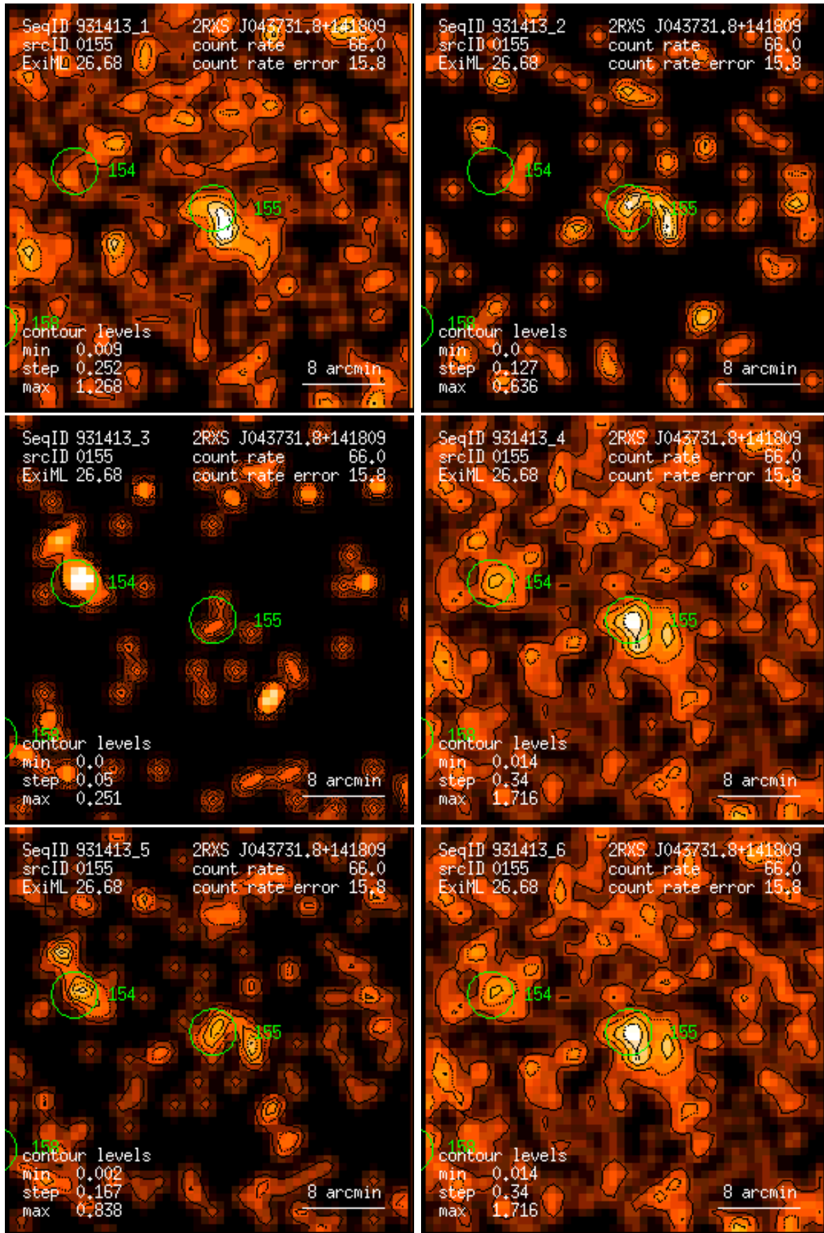
Figure 155: RASS 931413: detection 0155: band rate images, Gaussian filter: (1) PSPC channels 11 – 41, (2) 52 – 90, (3) 91 – 201, (4) 11 – 235, (5) 52 – 201, (6) 11 – 201. Broad band rates in counts/ks. Band rate contour levels in counts/ks/arcmin 2 .
