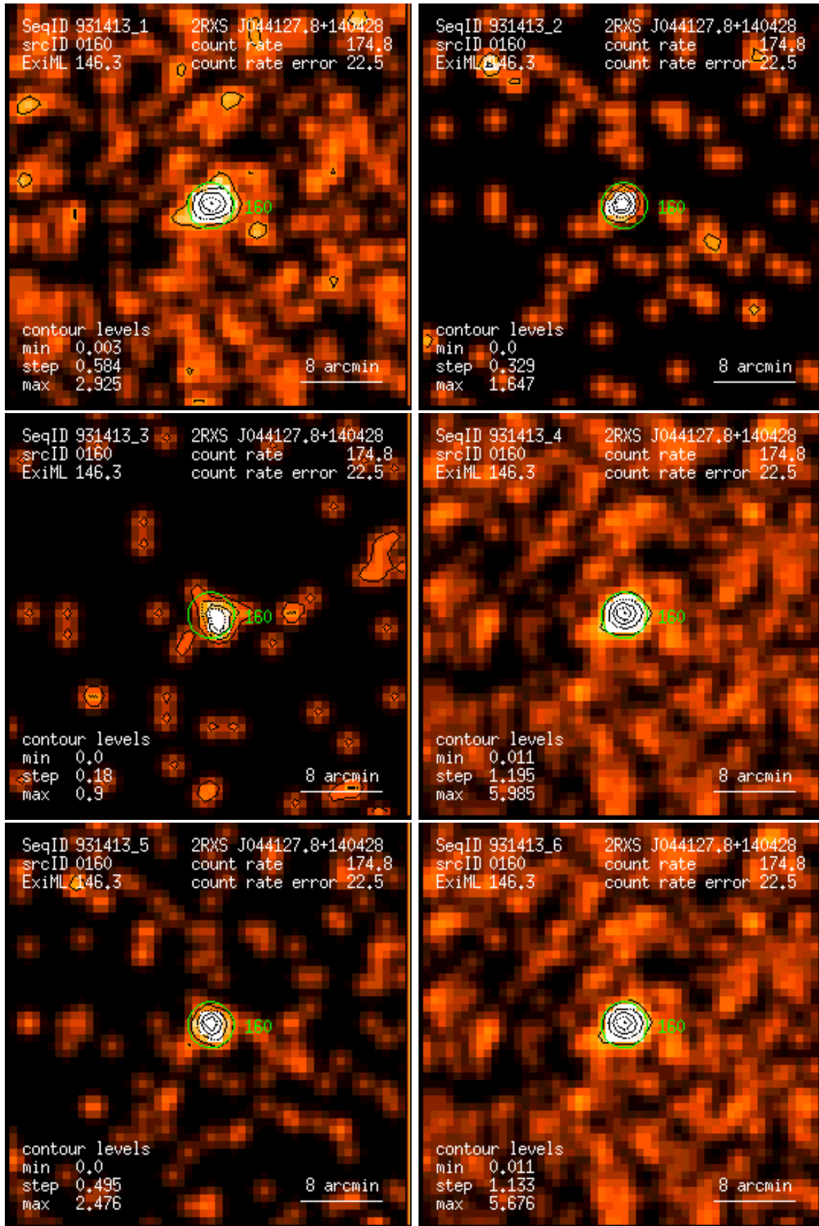
Figure 160: RASS 931413: detection 0160: band rate images, Gaussian filter: (1) PSPC channels 11 – 41, (2) 52 – 90, (3) 91 – 201, (4) 11 – 235, (5) 52 – 201, (6) 11 – 201. Broad band rates in counts/ks. Band rate contour levels in counts/ks/arcmin 2 .
