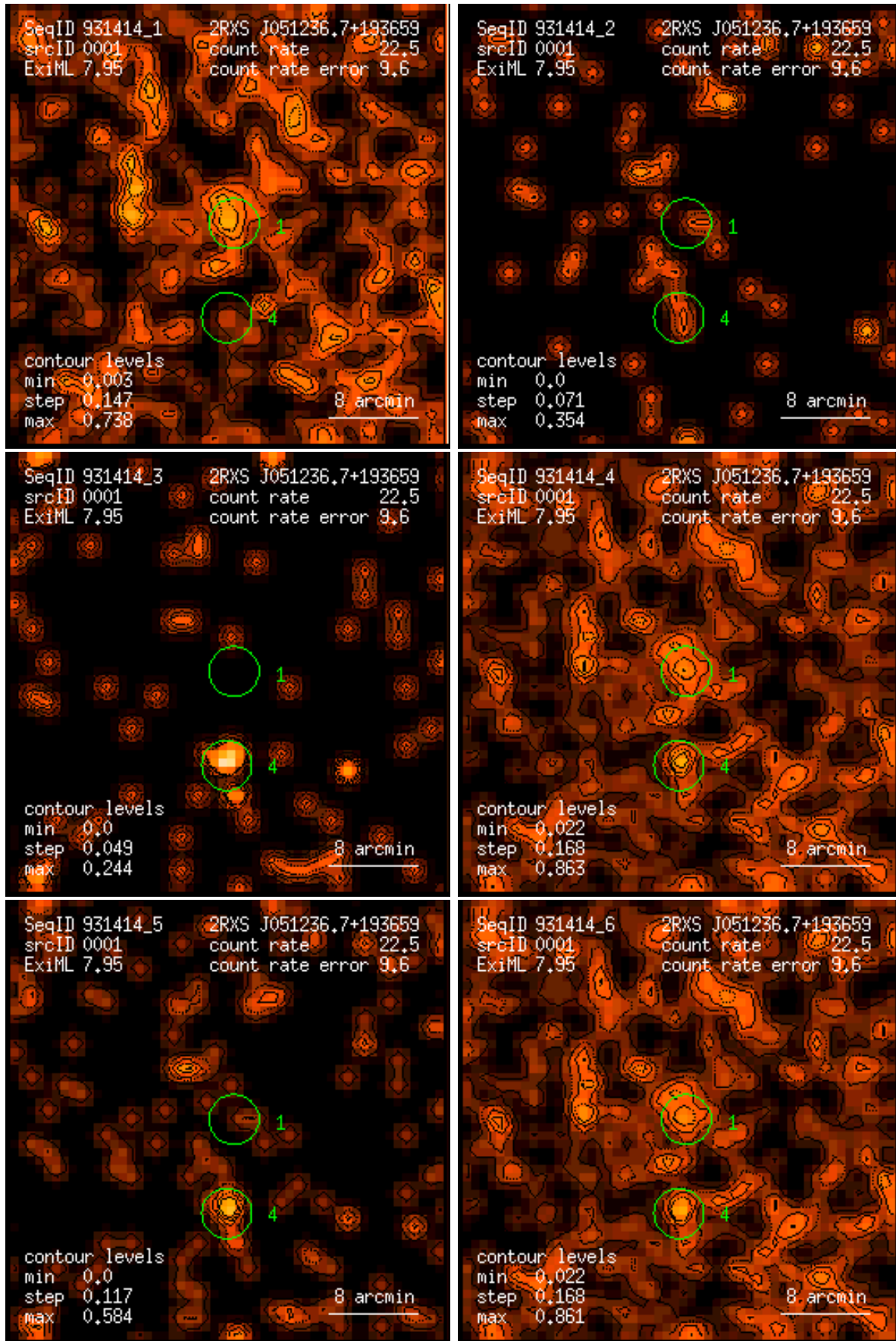
Figure 1: RASS 931414: detection 0001: band rate images, Gaussian filter: (1) PSPC channels 11 – 41, (2) 52 – 90, (3) 91 – 201, (4) 11 – 235, (5) 52 – 201, (6) 11 – 201. Broad band rates in counts/ks. Band rate contour levels in counts/ks/arcmin 2 .
