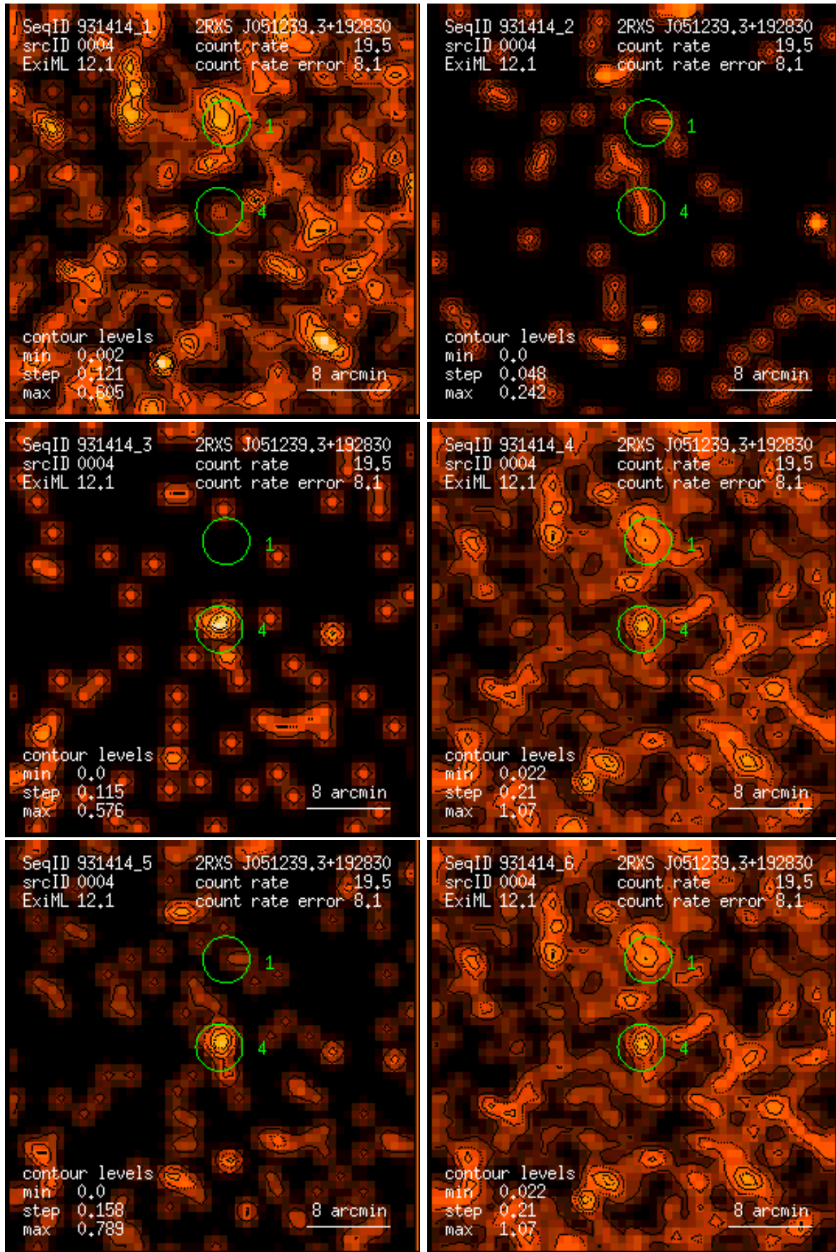
Figure 4: RASS 931414: detection 0004: band rate images, Gaussian filter: (1) PSPC channels 11 – 41, (2) 52 – 90, (3) 91 – 201, (4) 11 – 235, (5) 52 – 201, (6) 11 – 201. Broad band rates in counts/ks. Band rate contour levels in counts/ks/arcmin 2 .
