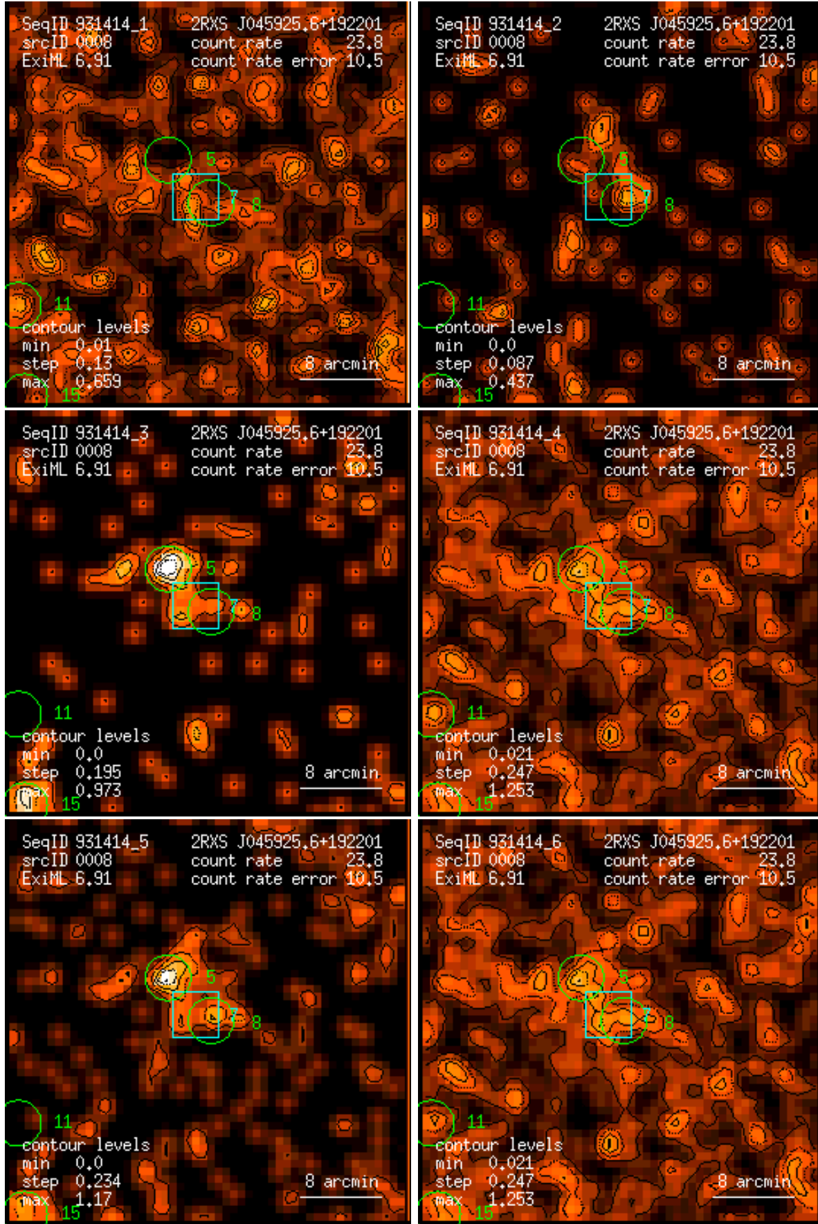
Figure 8: RASS 931414: detection 0008: band rate images, Gaussian filter: (1) PSPC channels 11 – 41, (2) 52 – 90, (3) 91 – 201, (4) 11 – 235, (5) 52 – 201, (6) 11 – 201. Broad band rates in counts/ks. Band rate contour levels in counts/ks/arcmin 2 .
