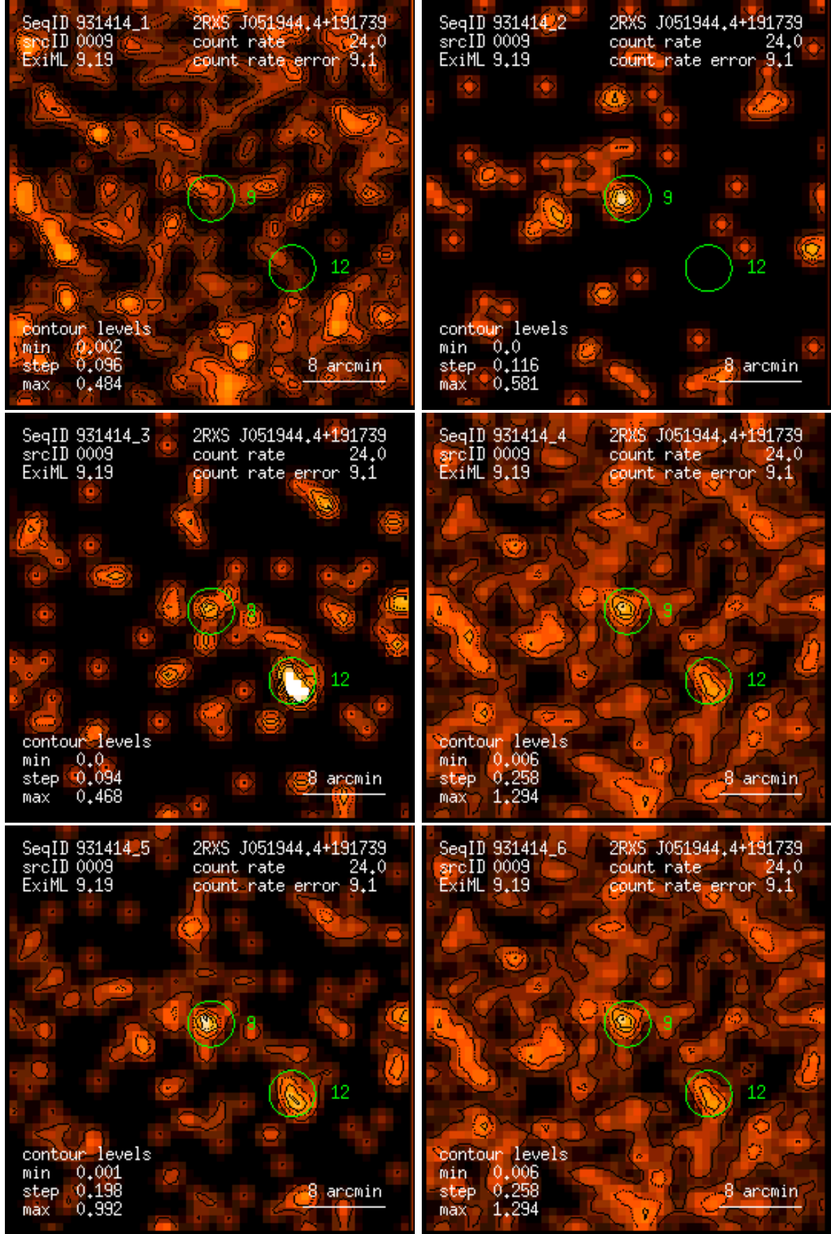
Figure 9: RASS 931414: detection 0009: band rate images, Gaussian filter: (1) PSPC channels 11 – 41, (2) 52 – 90, (3) 91 – 201, (4) 11 – 235, (5) 52 – 201, (6) 11 – 201. Broad band rates in counts/ks. Band rate contour levels in counts/ks/arcmin 2 .
