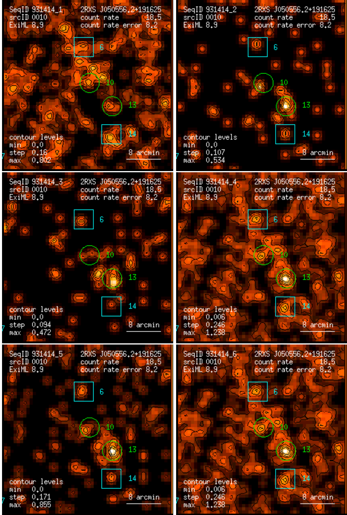
Figure 10: RASS 931414: detection 0010: band rate images, Gaussian filter: (1) PSPC channels 11 – 41, (2) 52 – 90, (3) 91 – 201, (4) 11 – 235, (5) 52 – 201, (6) 11 – 201. Broad band rates in counts/ks. Band rate contour levels in counts/ks/arcmin 2 .
