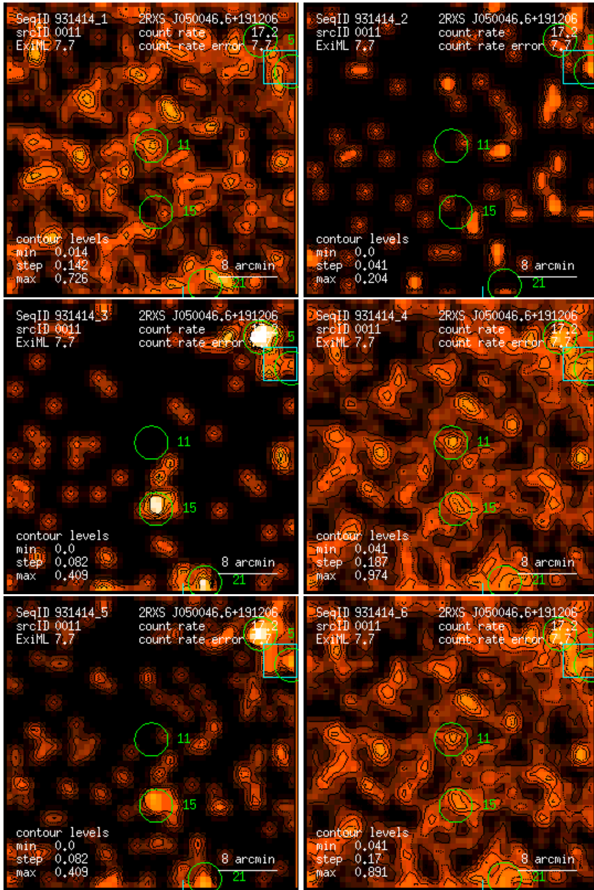
Figure 11: RASS 931414: detection 0011: band rate images, Gaussian filter: (1) PSPC channels 11 – 41, (2) 52 – 90, (3) 91 – 201, (4) 11 – 235, (5) 52 – 201, (6) 11 – 201. Broad band rates in counts/ks. Band rate contour levels in counts/ks/arcmin 2 .
