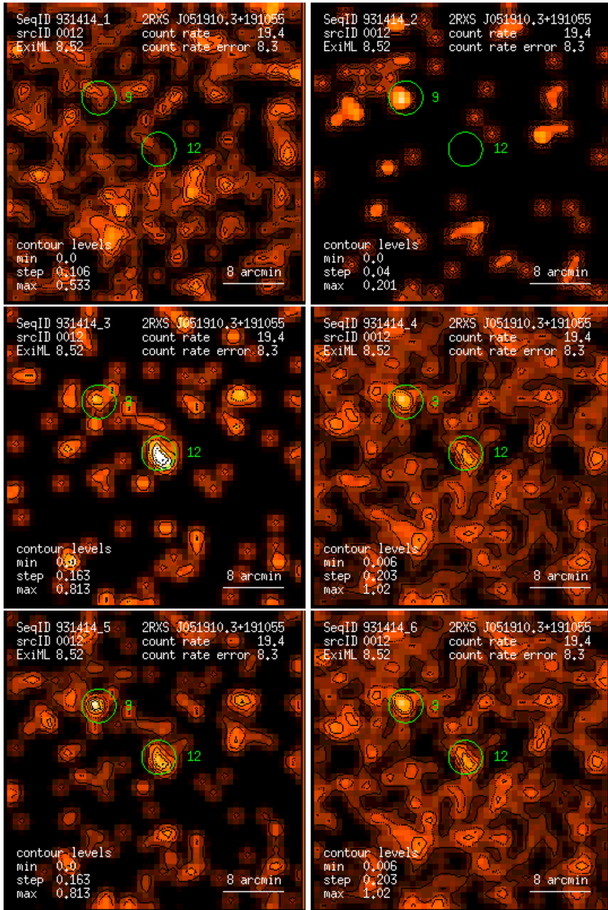
Figure 12: RASS 931414: detection 0012: band rate images, Gaussian filter: (1) PSPC channels 11 – 41, (2) 52 – 90, (3) 91 – 201, (4) 11 – 235, (5) 52 – 201, (6) 11 – 201. Broad band rates in counts/ks. Band rate contour levels in counts/ks/arcmin 2 .
