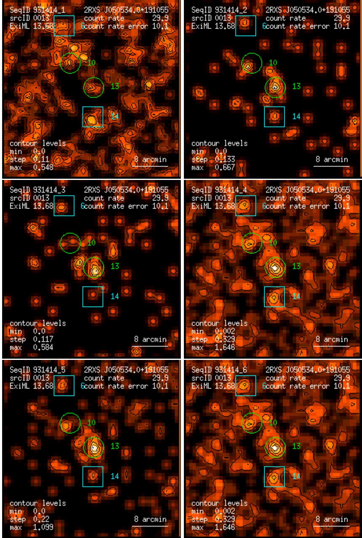
Figure 13: RASS 931414: detection 0013: band rate images, Gaussian filter: (1) PSPC channels 11 – 41, (2) 52 – 90, (3) 91 – 201, (4) 11 – 235, (5) 52 – 201, (6) 11 – 201. Broad band rates in counts/ks. Band rate contour levels in counts/ks/arcmin 2 .
