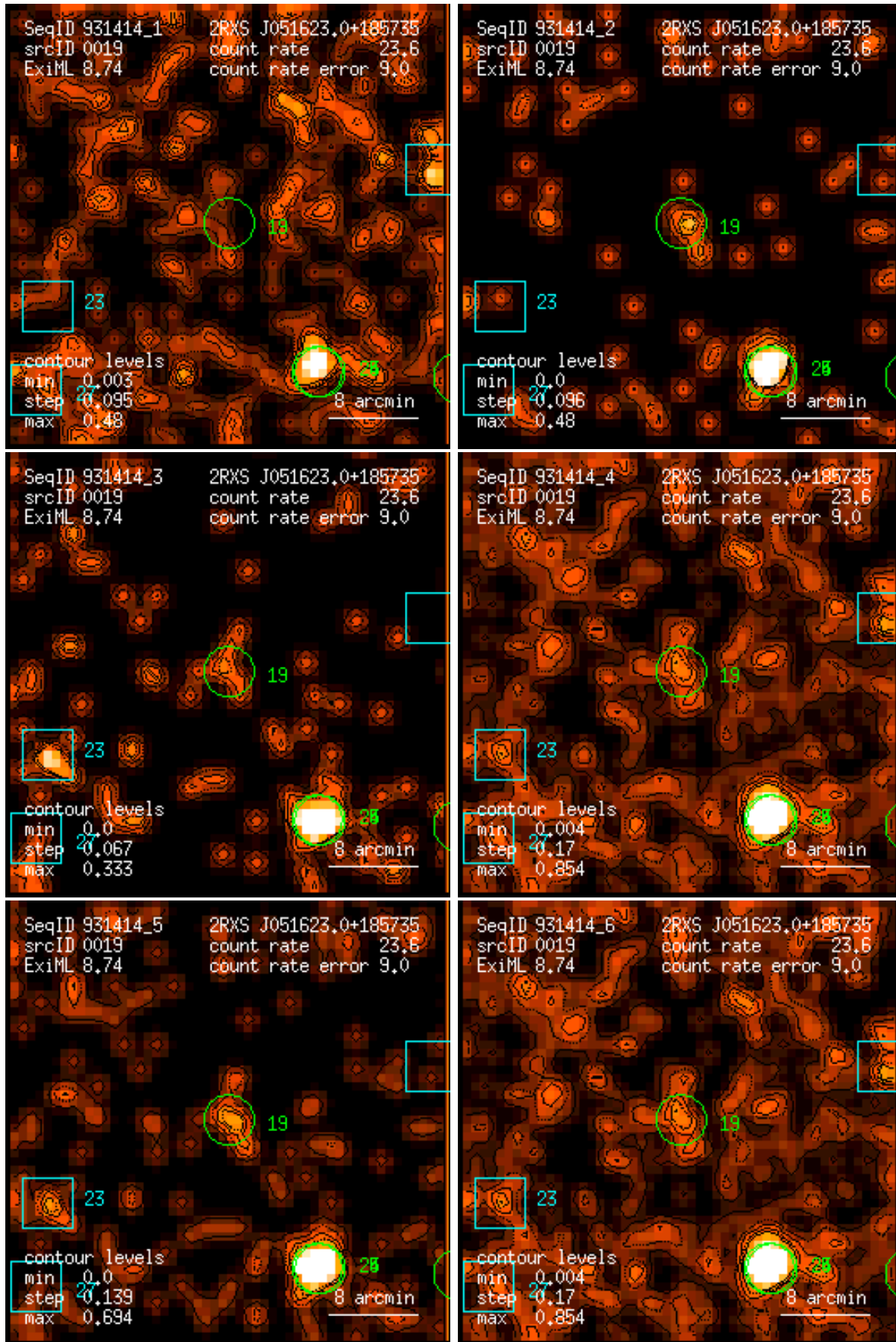
Figure 19: RASS 931414: detection 0019: band rate images, Gaussian filter: (1) PSPC channels 11 – 41, (2) 52 – 90, (3) 91 – 201, (4) 11 – 235, (5) 52 – 201, (6) 11 – 201. Broad band rates in counts/ks. Band rate contour levels in counts/ks/arcmin 2 .
