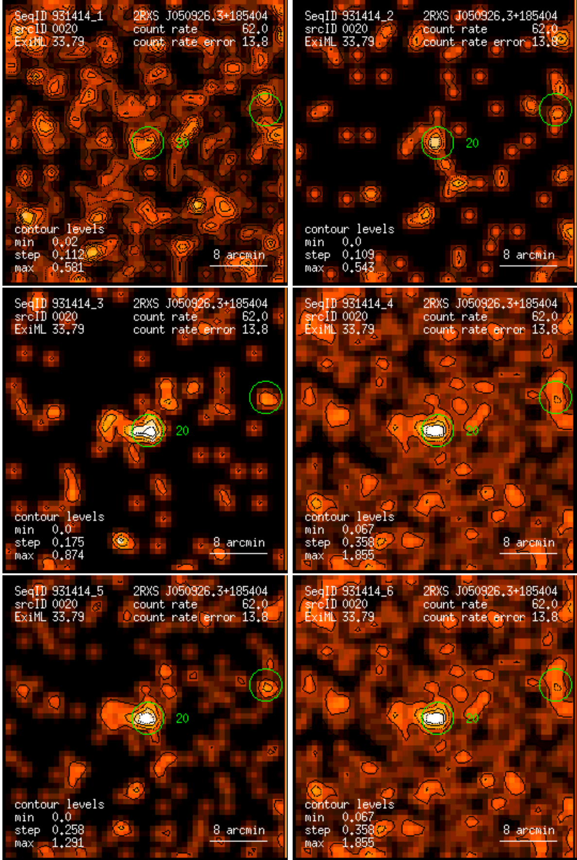
Figure 20: RASS 931414: detection 0020: band rate images, Gaussian filter: (1) PSPC channels 11 – 41, (2) 52 – 90, (3) 91 – 201, (4) 11 – 235, (5) 52 – 201, (6) 11 – 201. Broad band rates in counts/ks. Band rate contour levels in counts/ks/arcmin 2 .
