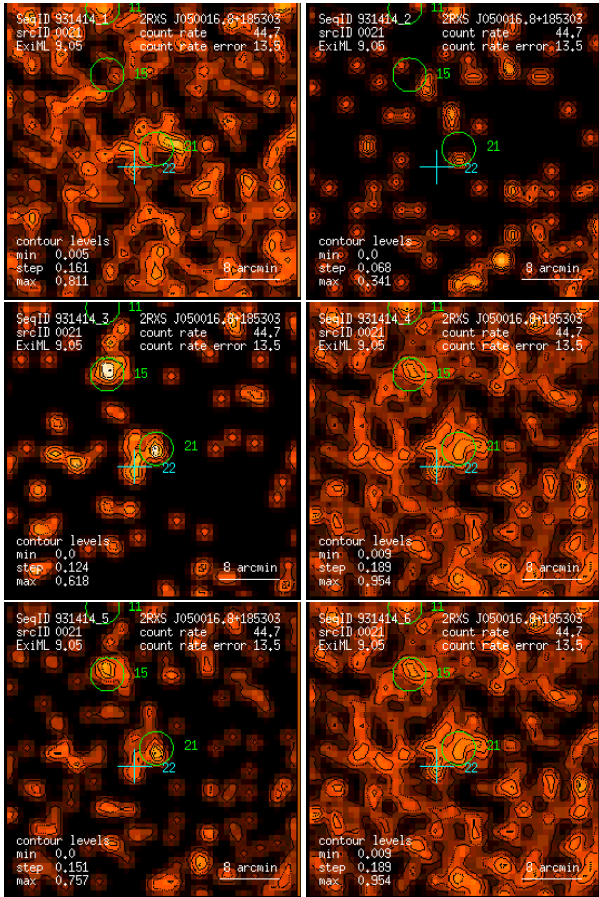
Figure 21: RASS 931414: detection 0021: band rate images, Gaussian filter: (1) PSPC channels 11 – 41, (2) 52 – 90, (3) 91 – 201, (4) 11 – 235, (5) 52 – 201, (6) 11 – 201. Broad band rates in counts/ks. Band rate contour levels in counts/ks/arcmin 2 .
