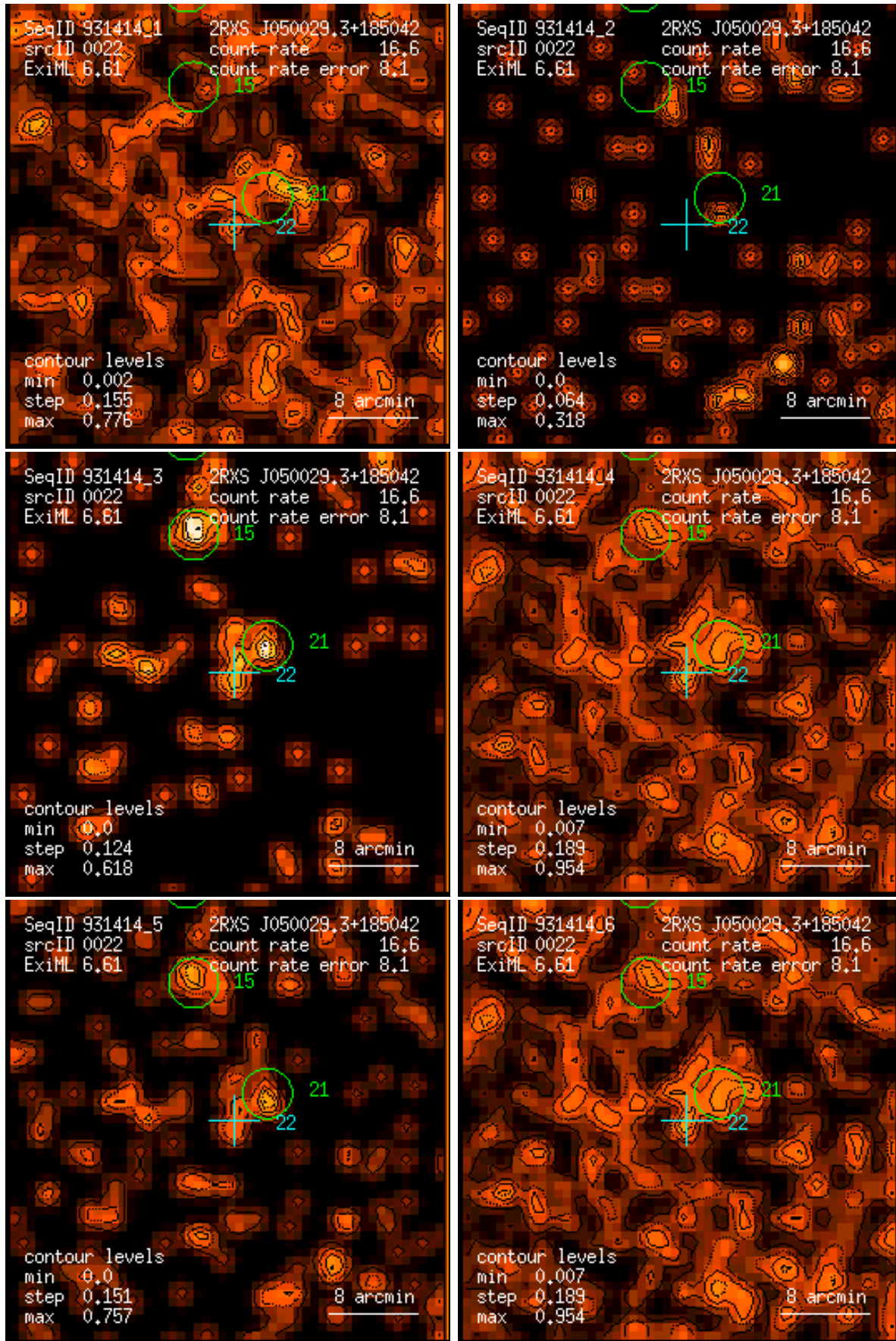
Figure 22: RASS 931414: detection 0022: band rate images, Gaussian filter: (1) PSPC channels 11 – 41, (2) 52 – 90, (3) 91 – 201, (4) 11 – 235, (5) 52 – 201, (6) 11 – 201. Broad band rates in counts/ks. Band rate contour levels in counts/ks/arcmin 2 .
