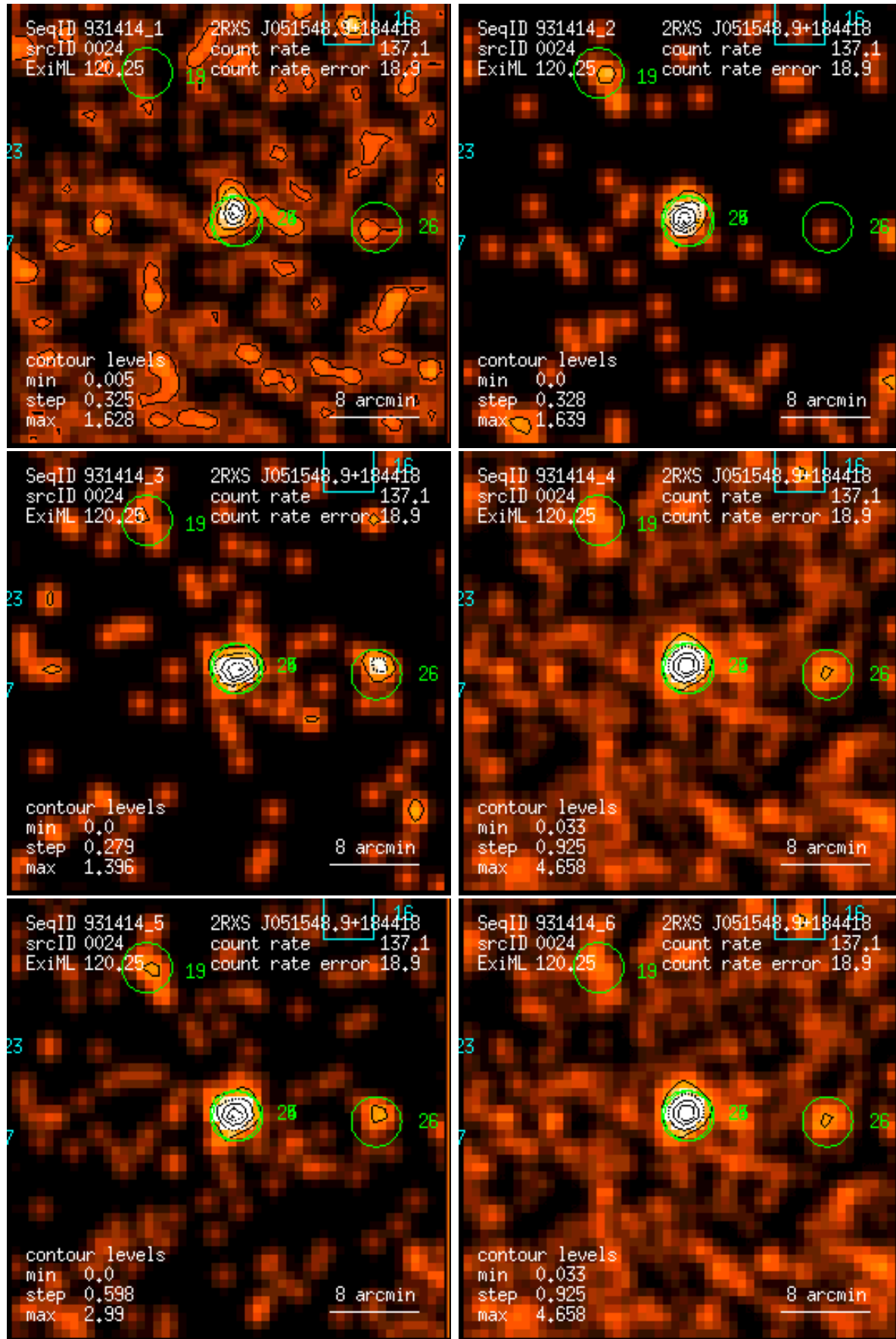
Figure 24: RASS 931414: detection 0024: band rate images, Gaussian filter: (1) PSPC channels 11 – 41, (2) 52 – 90, (3) 91 – 201, (4) 11 – 235, (5) 52 – 201, (6) 11 – 201. Broad band rates in counts/ks. Band rate contour levels in counts/ks/arcmin 2 .
