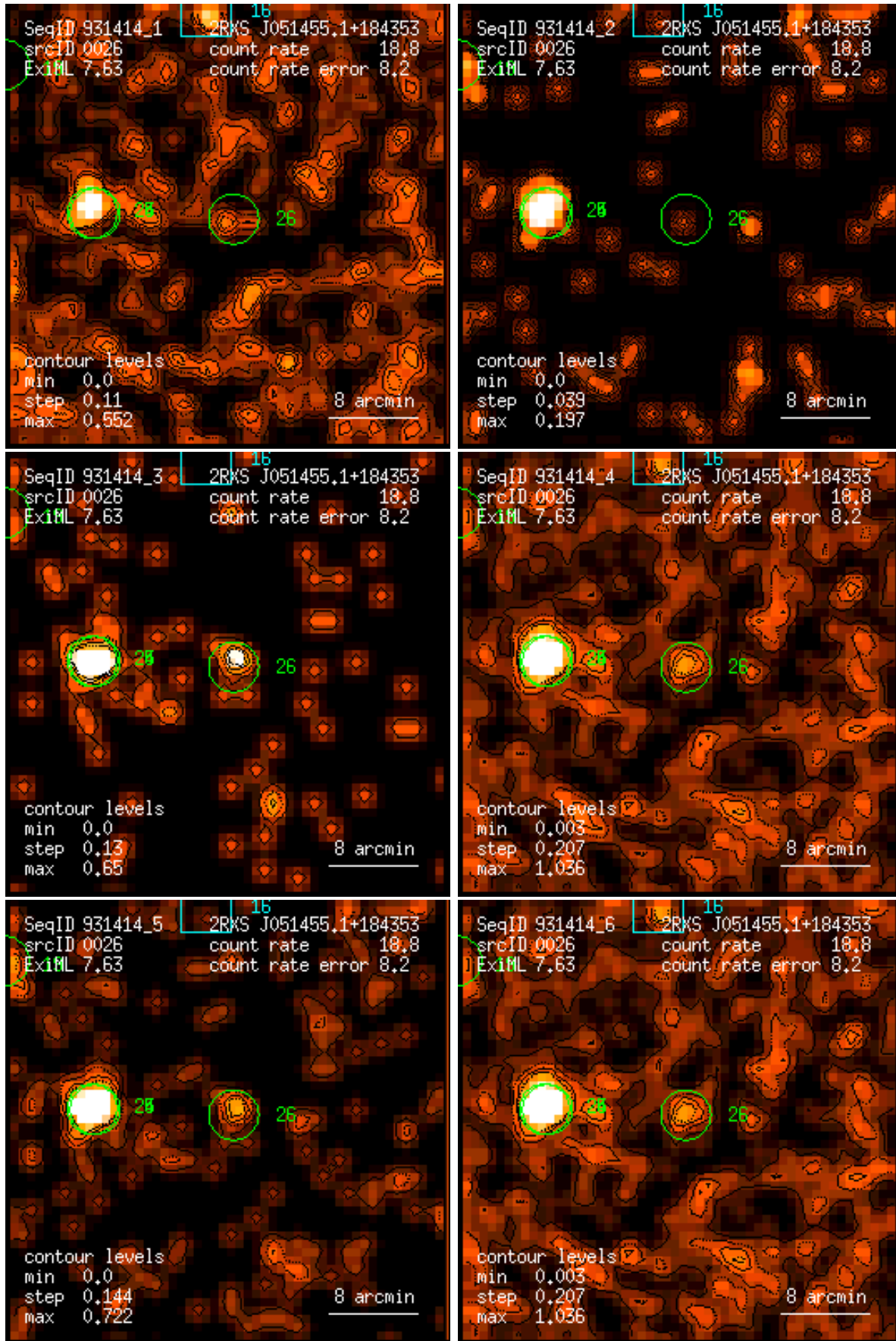
Figure 26: RASS 931414: detection 0026: band rate images, Gaussian filter: (1) PSPC channels 11 – 41, (2) 52 – 90, (3) 91 – 201, (4) 11 – 235, (5) 52 – 201, (6) 11 – 201. Broad band rates in counts/ks. Band rate contour levels in counts/ks/arcmin 2 .
