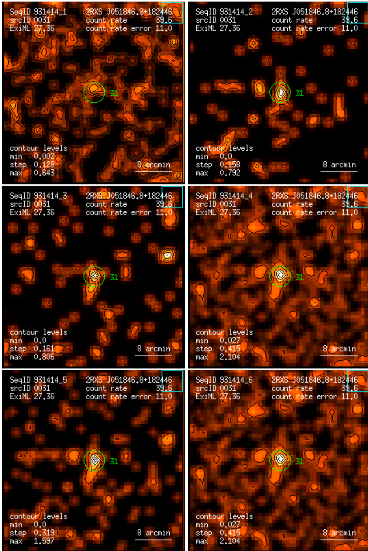
Figure 31: RASS 931414: detection 0031: band rate images, Gaussian filter: (1) PSPC channels 11 – 41, (2) 52 – 90, (3) 91 – 201, (4) 11 – 235, (5) 52 – 201, (6) 11 – 201. Broad band rates in counts/ks. Band rate contour levels in counts/ks/arcmin 2 .
