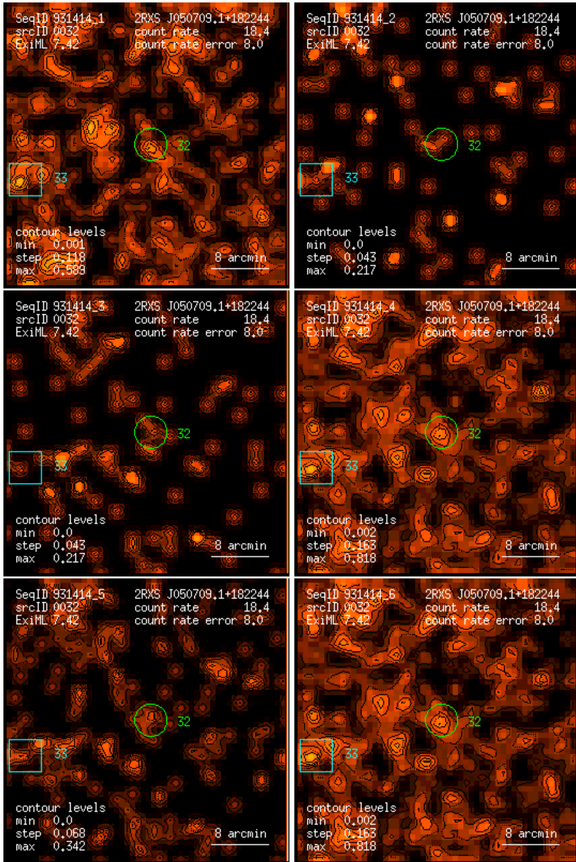
Figure 32: RASS 931414: detection 0032: band rate images, Gaussian filter: (1) PSPC channels 11 – 41, (2) 52 – 90, (3) 91 – 201, (4) 11 – 235, (5) 52 – 201, (6) 11 – 201. Broad band rates in counts/ks. Band rate contour levels in counts/ks/arcmin 2 .
