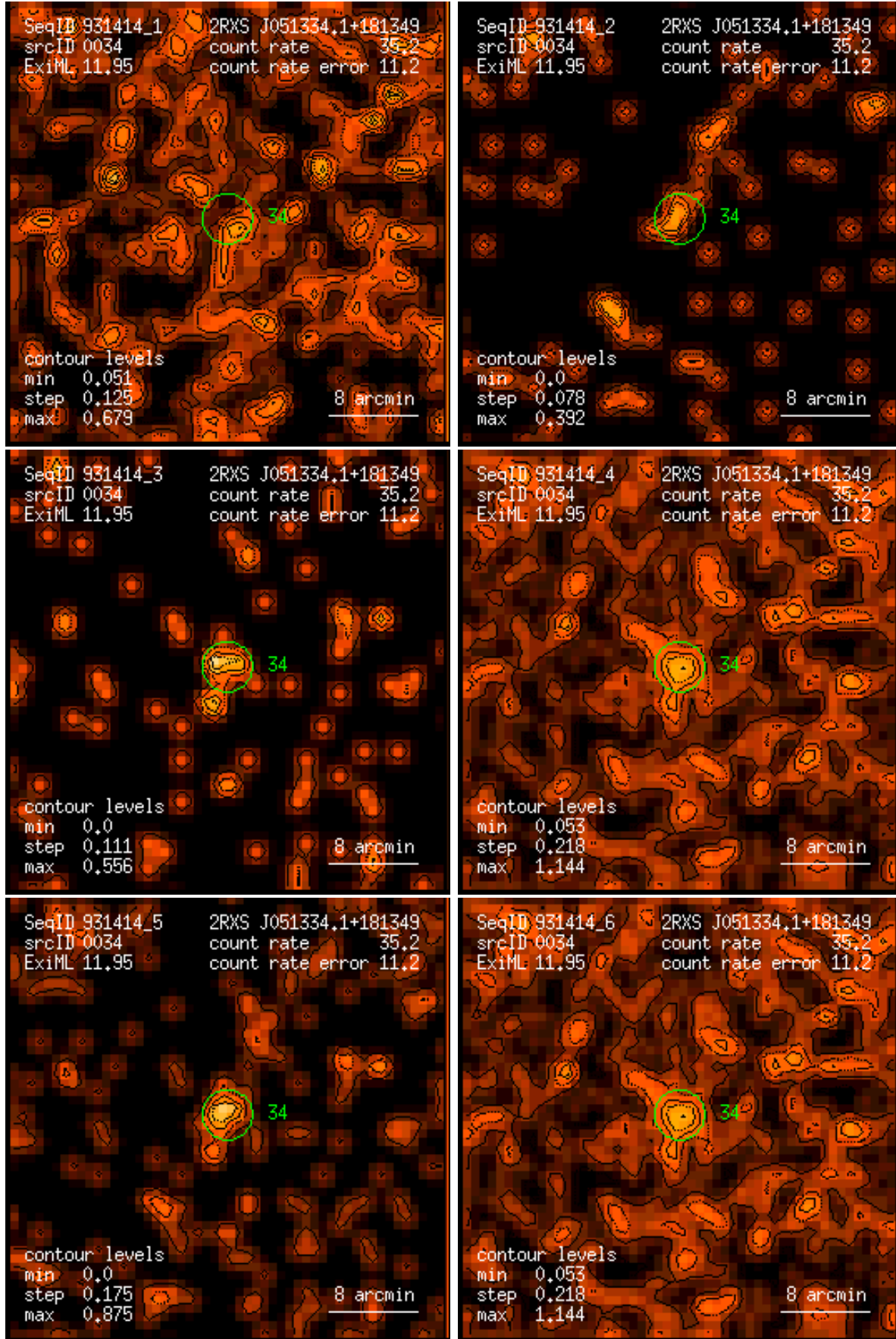
Figure 34: RASS 931414: detection 0034: band rate images, Gaussian filter: (1) PSPC channels 11 – 41, (2) 52 – 90, (3) 91 – 201, (4) 11 – 235, (5) 52 – 201, (6) 11 – 201. Broad band rates in counts/ks. Band rate contour levels in counts/ks/arcmin 2 .
