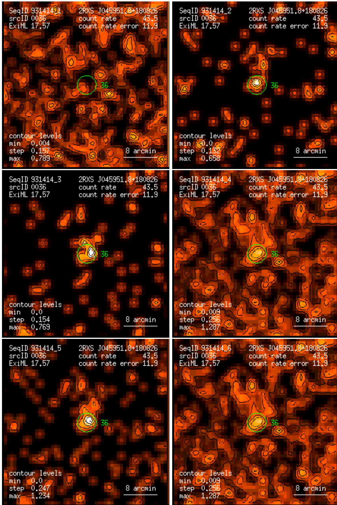
Figure 36: RASS 931414: detection 0036: band rate images, Gaussian filter: (1) PSPC channels 11 – 41, (2) 52 – 90, (3) 91 – 201, (4) 11 – 235, (5) 52 – 201, (6) 11 – 201. Broad band rates in counts/ks. Band rate contour levels in counts/ks/arcmin 2 .
