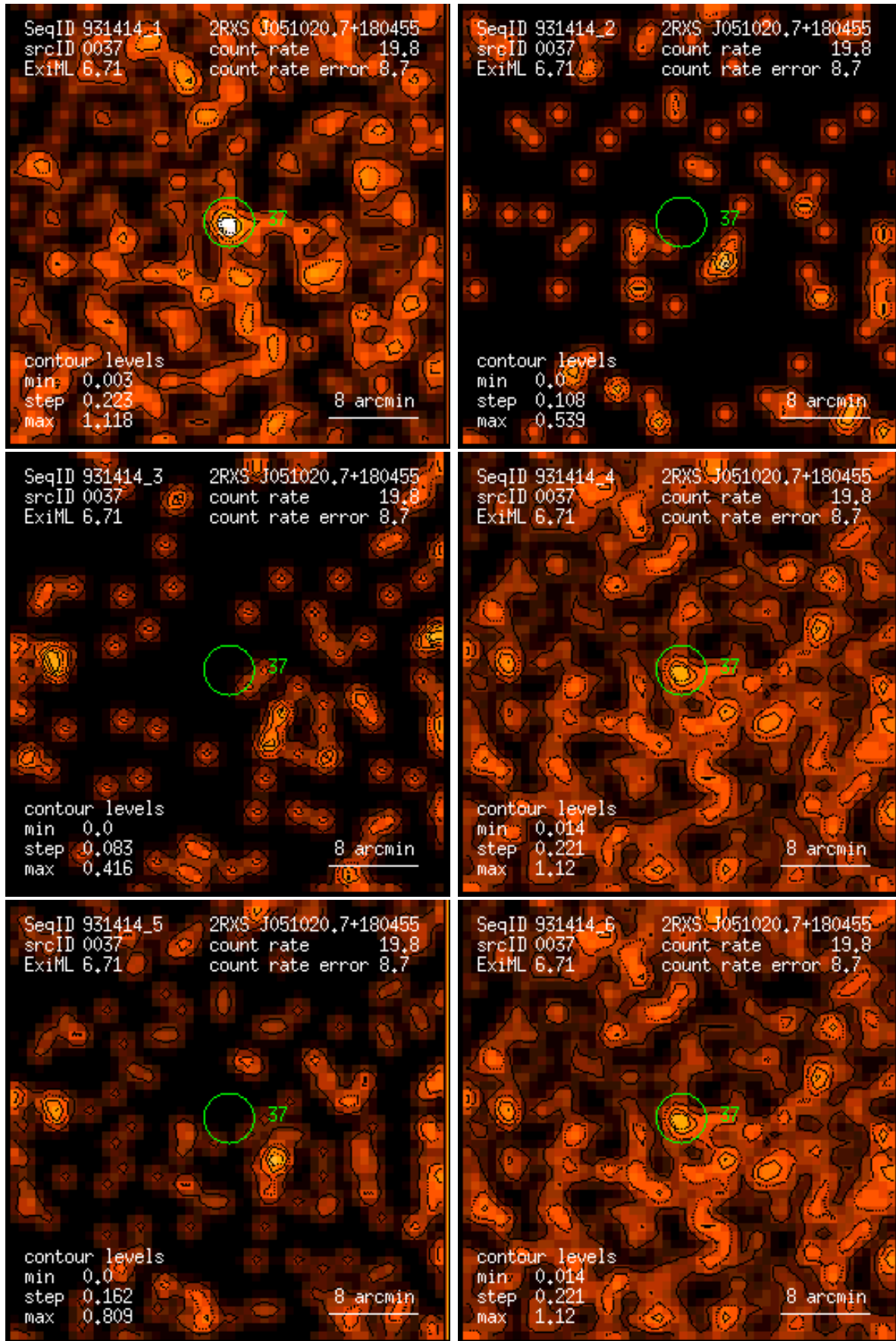
Figure 37: RASS 931414: detection 0037: band rate images, Gaussian filter: (1) PSPC channels 11 – 41, (2) 52 – 90, (3) 91 – 201, (4) 11 – 235, (5) 52 – 201, (6) 11 – 201. Broad band rates in counts/ks. Band rate contour levels in counts/ks/arcmin 2 .
