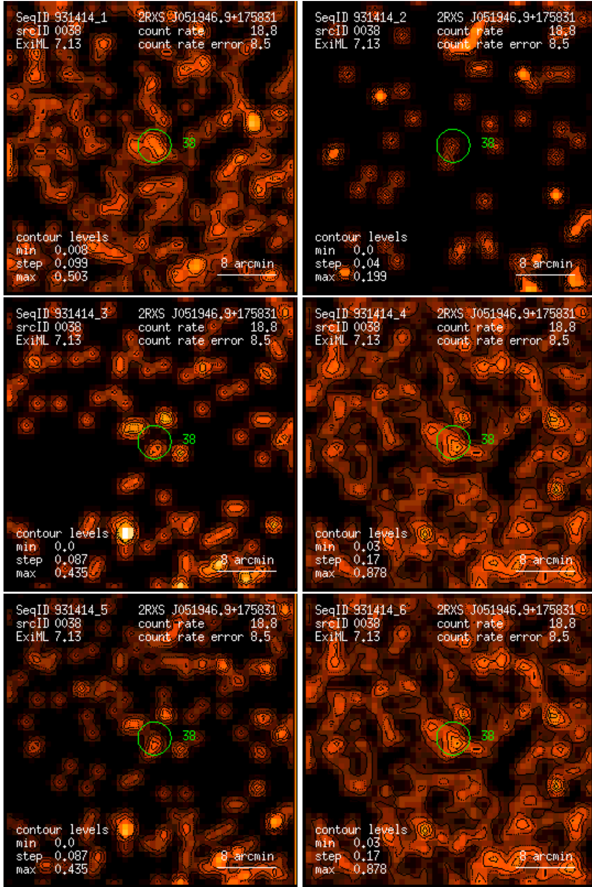
Figure 38: RASS 931414: detection 0038: band rate images, Gaussian filter: (1) PSPC channels 11 – 41, (2) 52 – 90, (3) 91 – 201, (4) 11 – 235, (5) 52 – 201, (6) 11 – 201. Broad band rates in counts/ks. Band rate contour levels in counts/ks/arcmin 2 .
