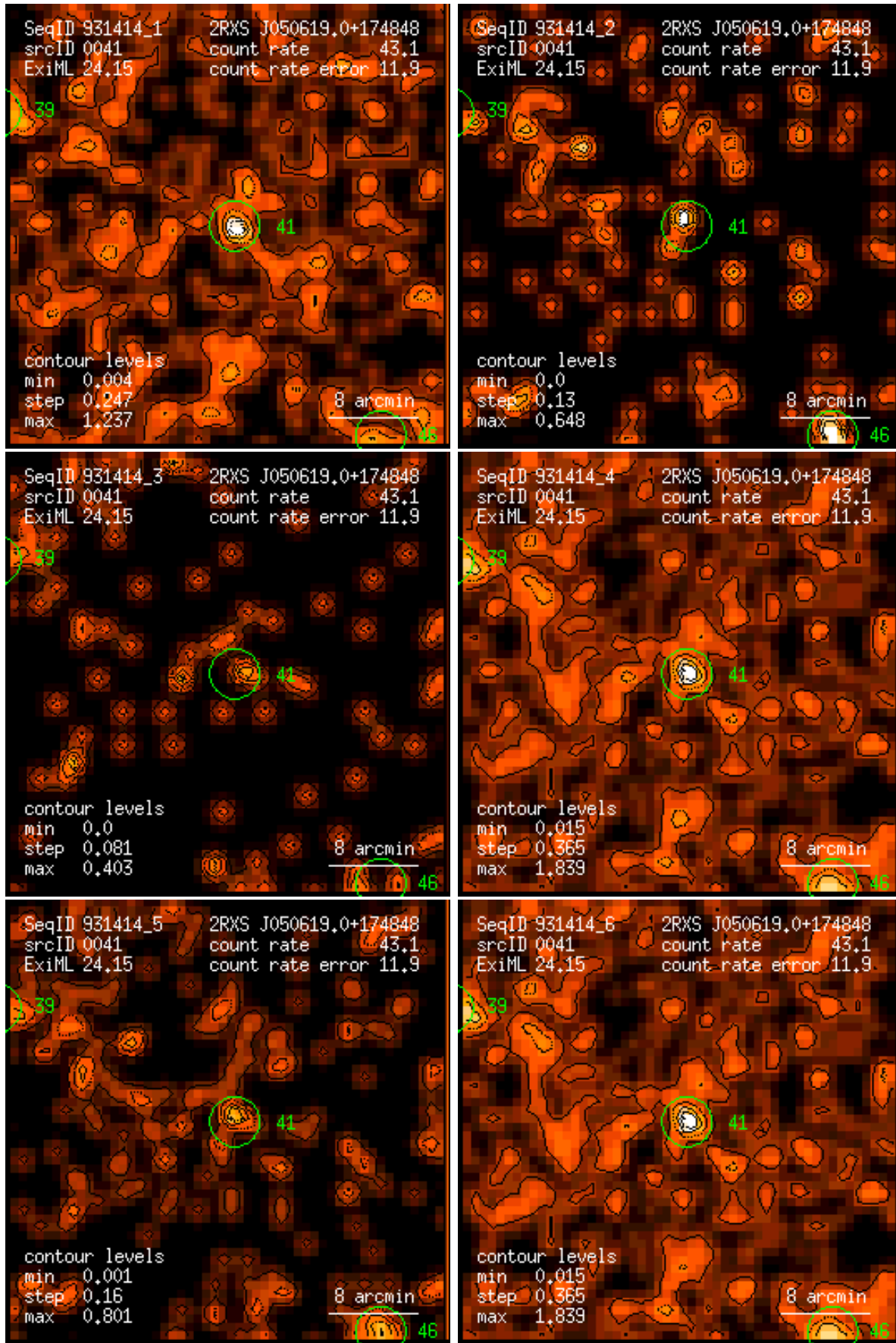
Figure 41: RASS 931414: detection 0041: band rate images, Gaussian filter: (1) PSPC channels 11 – 41, (2) 52 – 90, (3) 91 – 201, (4) 11 – 235, (5) 52 – 201, (6) 11 – 201. Broad band rates in counts/ks. Band rate contour levels in counts/ks/arcmin 2 .
